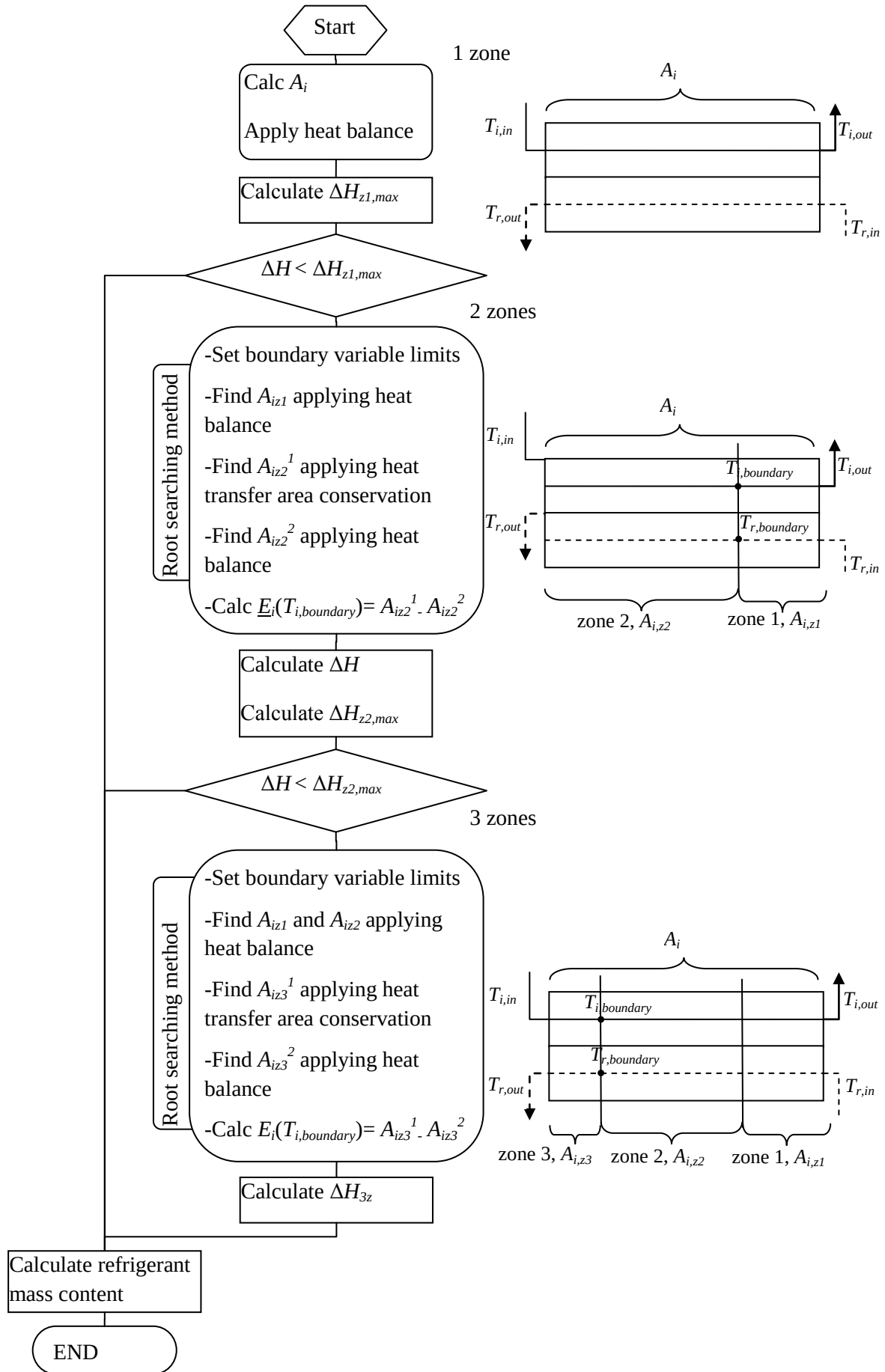
Fig. 2. Generic adaptive zone heat exchanger model
