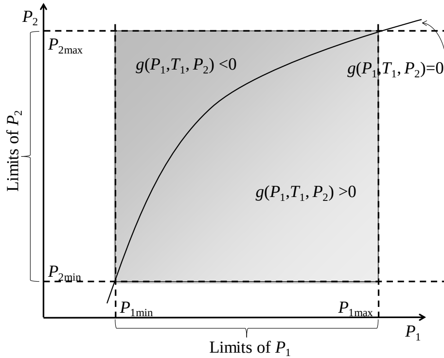
b) The limits for the suction pressure P_1 are set according to the limits of the discharge pressure P_2 . The function g expresses the difference between the mass flow rate calculated by each regulation device in the cycle. The solution for P_1 , T_1 , and P_2 represents a point that must exist on the line g within the shaded region
