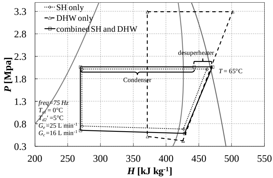
Fig. 9. Simulation results for the compact GSHP with a desuperheater for three of its operation modes under the same climate conditions
