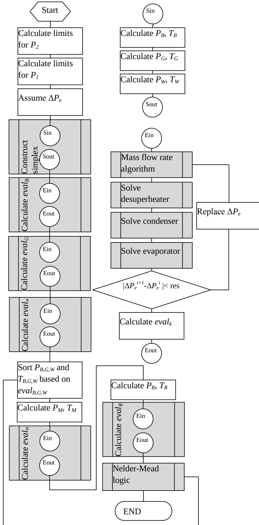
Fig. 4. Global convergence algorithm
