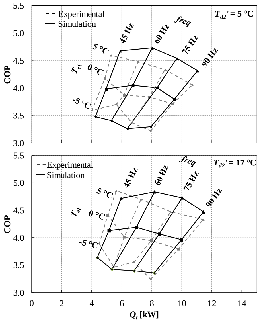
Fig. 8. Comparison of mapping results for T_{d2}' = 5^\circ\text{C} and 17^\circ\text{C} between experimental and simulation results
