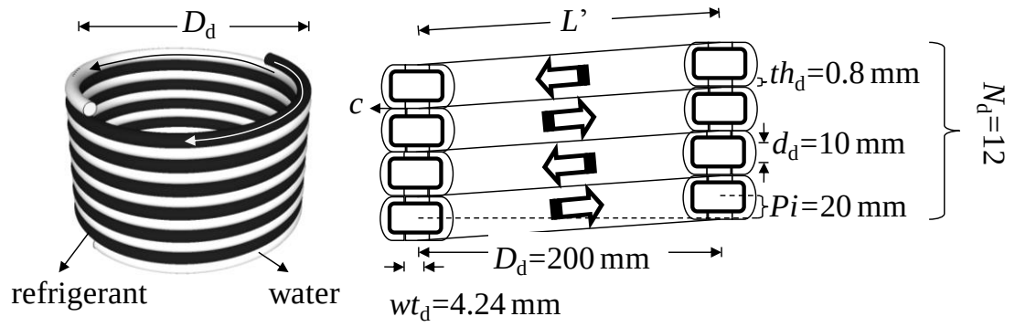
a). Indirect contact coil type desuperheater
