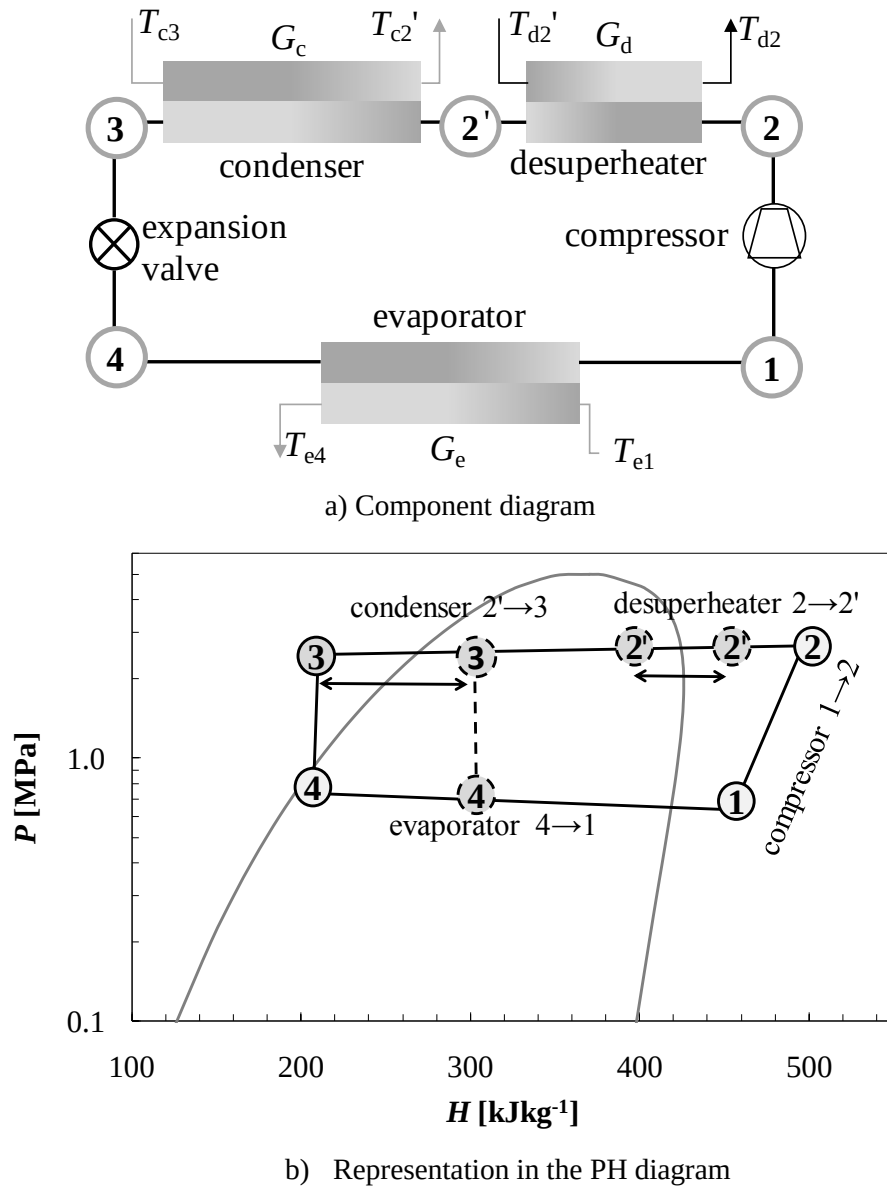
Fig. 1. Compact GSHP with desuperheater
