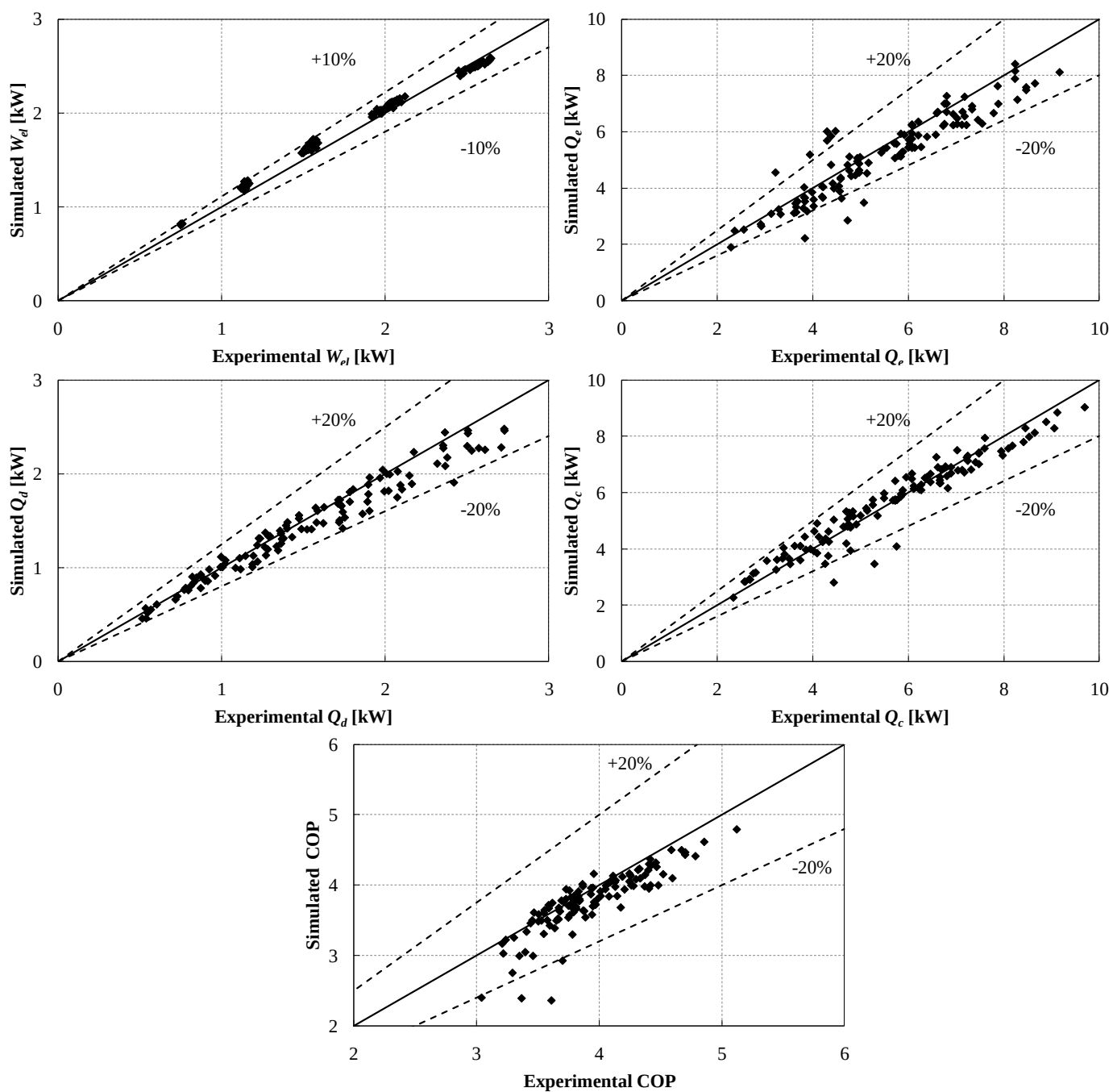
Fig. 6. Complete system comparison between experimental and simulation results
