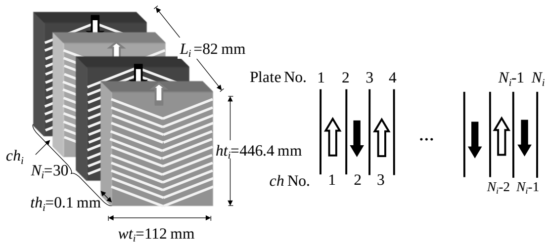
b) Condenser and evaporator plate type heat exchangers
