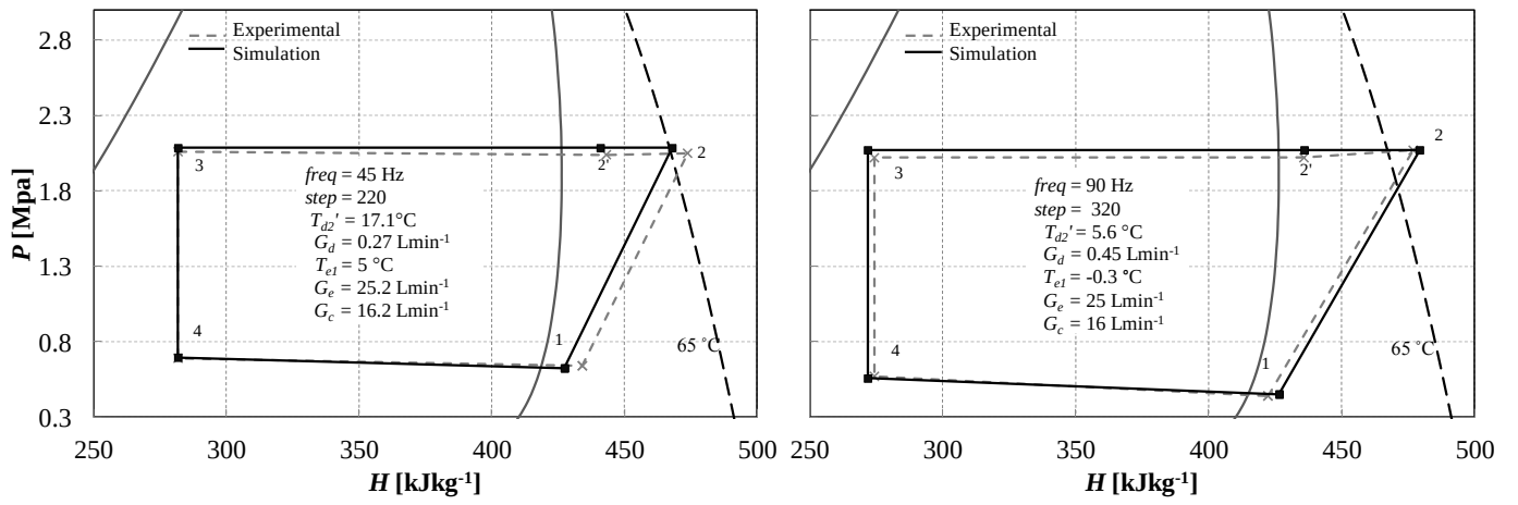
Fig. 7. Comparison between simulated and experimental refrigeration cycles in the PH diagram.
