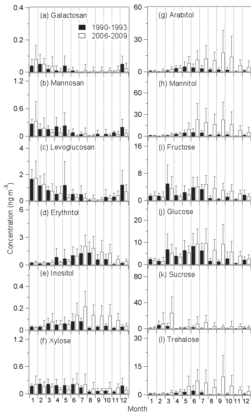
Figure 6. Monthly averaged concentrations of saccharides in the marine aerosols collected from Chichi-Jima Island. Error bars represent the standard deviation.
