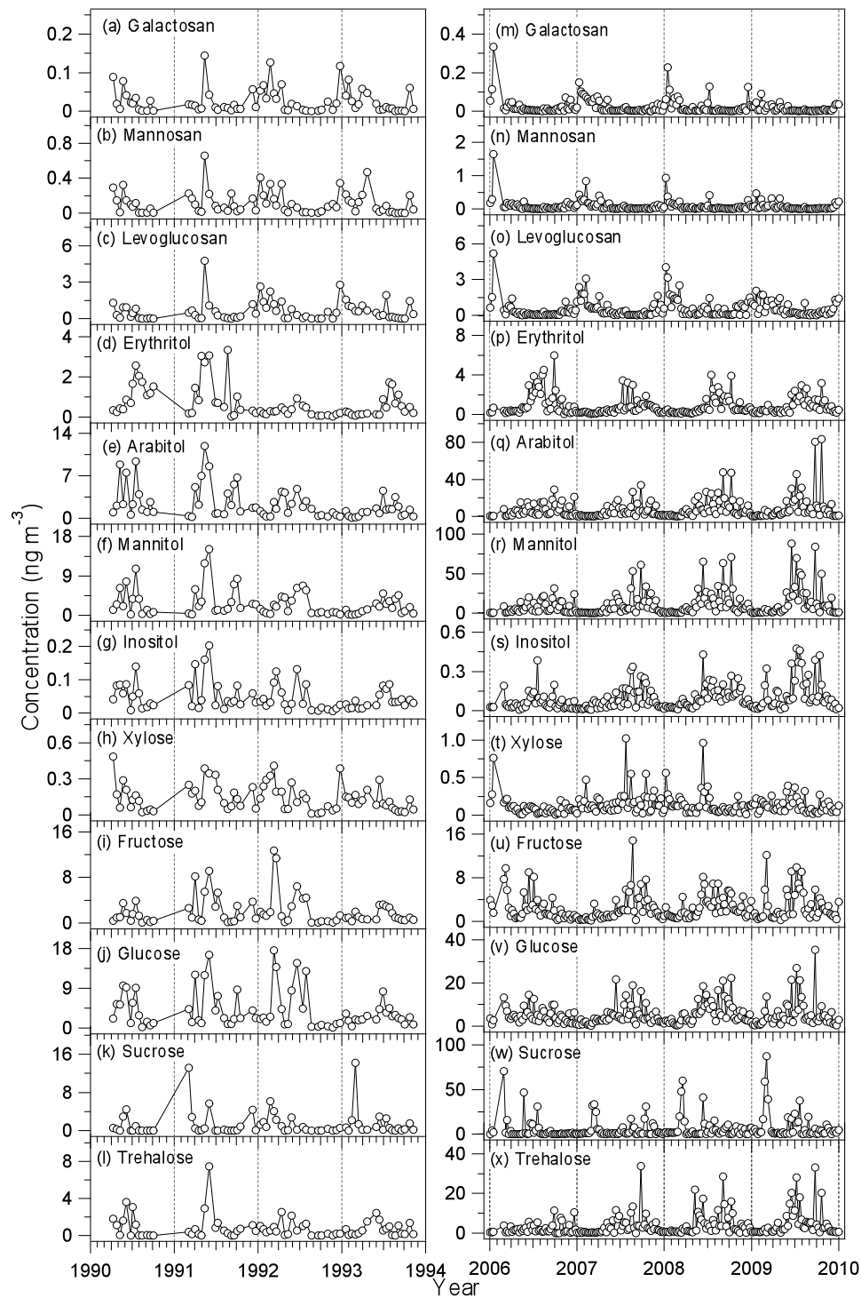
Figure 4. Temporal variations of anhydrosugars (galactosan, mannosan and levoglucosan), sugar alcohols (erythritol, arabitrol, mannitol and inositol), and sugars (xylose, fructose, glucose, sucrose and trehalose) in the marine aerosols from Chichi-Jima Island, the western North Pacific.
