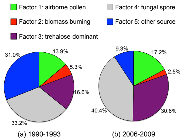
Figure 8. Pie diagrams showing the estimated average contributions of the five factors resolved by PMF to the measured saccharide compounds in the Chichi-Jima aerosol samples.
