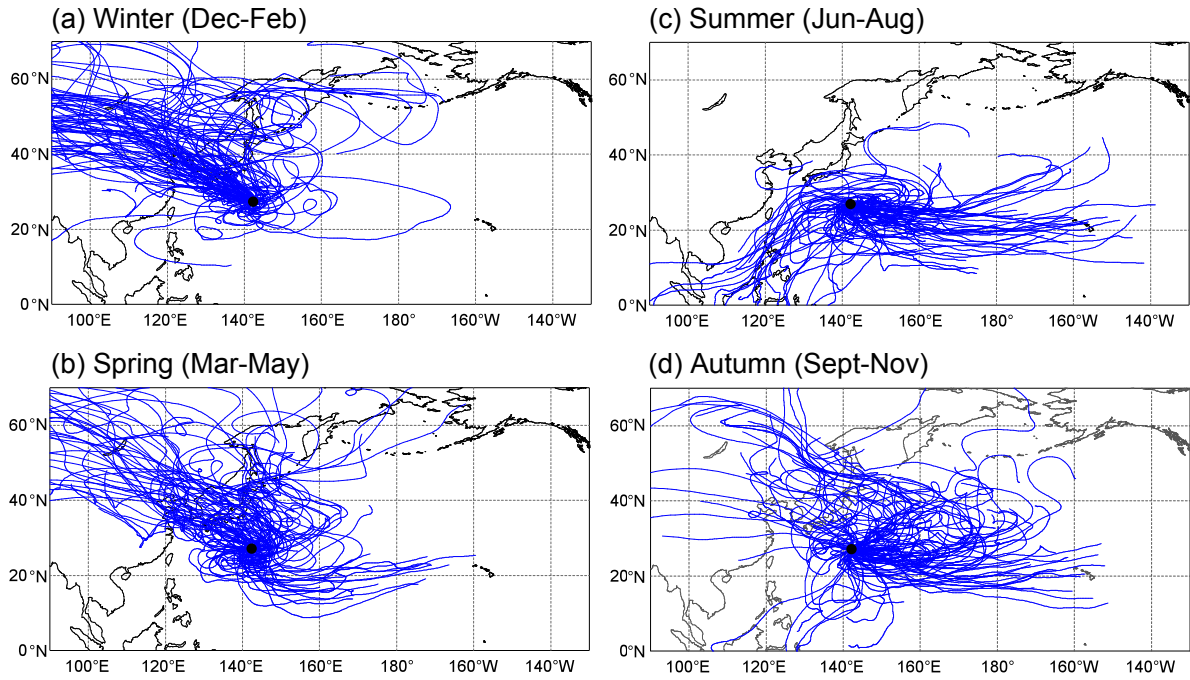
Figure 5. Ten-day back trajectories of air masses that arrived over the Chichi-Jima Island in (a) winter (December 2008-February 2009), (b) spring (March-May, 2009), (c) summer (June-August, 2009), and (d) autumn (September-November, 2009). The trajectories were calculated every 24 h at 12:00 (Local Time).
