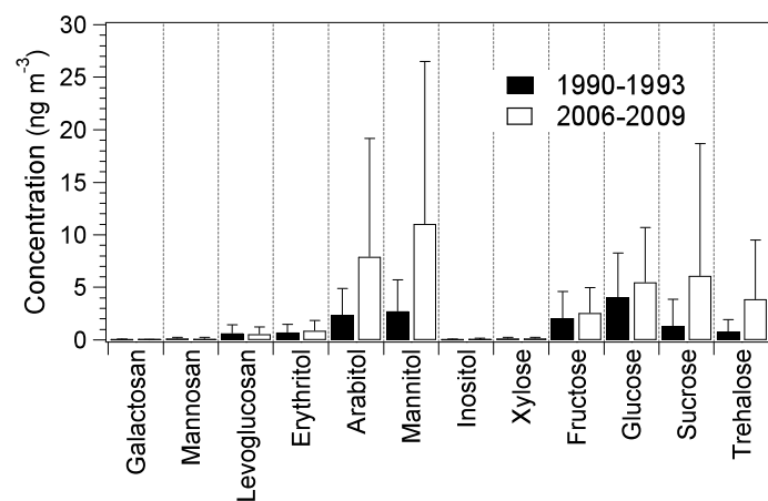
Figure 2. Averaged concentrations of saccharides in atmospheric aerosols collected at Chichi-Jima Island in the western North Pacific during the 1990-1993 and 2006-2009 periods. Error bars represent the standard deviation.
