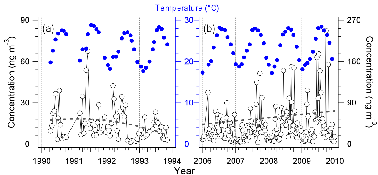
Figure 3. Temporal variations in the concentrations of total saccharides measured in the marine aerosols collected from Chichi-Jima Island, the western North Pacific during (a) 1990-1993, and (b) 2006-2009. The monthly-averaged ambient temperatures are present in the figure.
