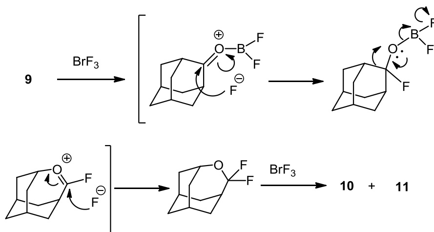
Scheme 1. Plausible mechanism for the formation of 10 and 11
