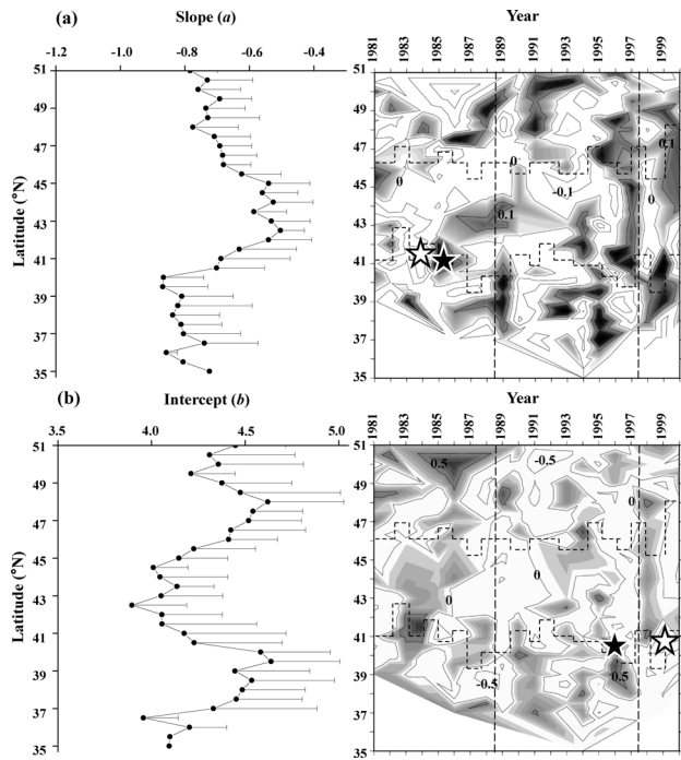
Fig. 7. Latitudinal changes in the mean and standard deviation (left) and anomalies (right) of the slope (a) and intercept (b) of the NBSS ( Y=aX+b ) on mesozooplankton biomass along the 180° line in the central North Pacific during June of 1981–2000. For panels on the right, the positions of water mass boundaries and periods of climate regime shifts (cf. Fig. 2) are superimposed. Solid and open stars indicate maximum and minimum values of the anomaly, respectively.
