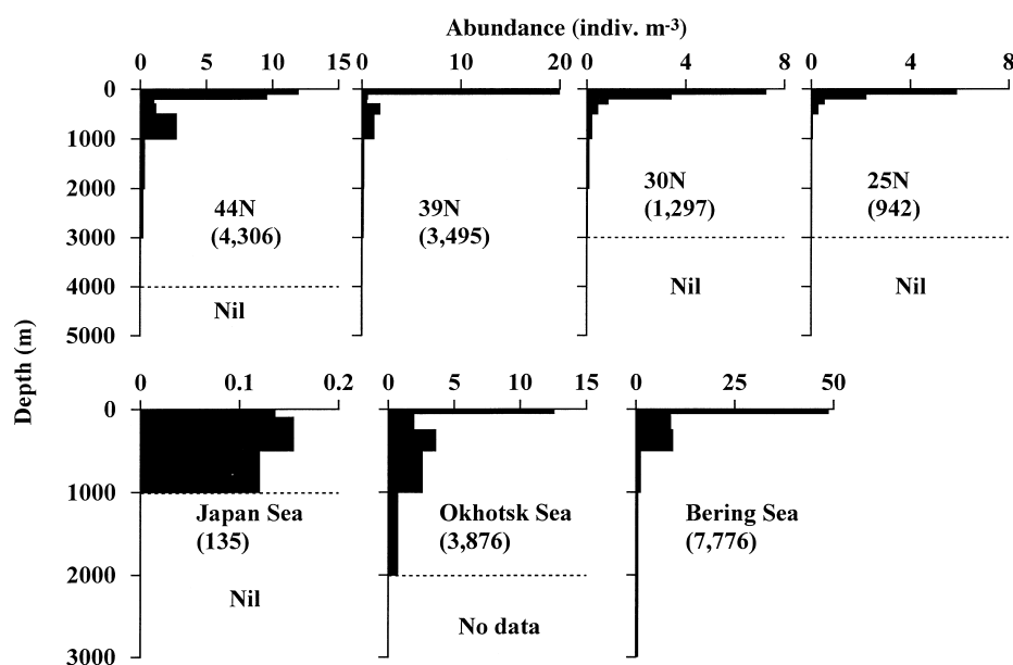
Fig. 3. Vertical distribution of the abundance of chaetognaths (indiv. m -3 ) at four stations in the western North Pacific Ocean (upper) and at single stations in the Japan Sea, Okhotsk Sea, and Bering Sea (lower). Note that abundance scales vary between panels. Water column integrated standing stocks (indiv. m -2 ) are shown in parentheses. Nil: no occurrence.
