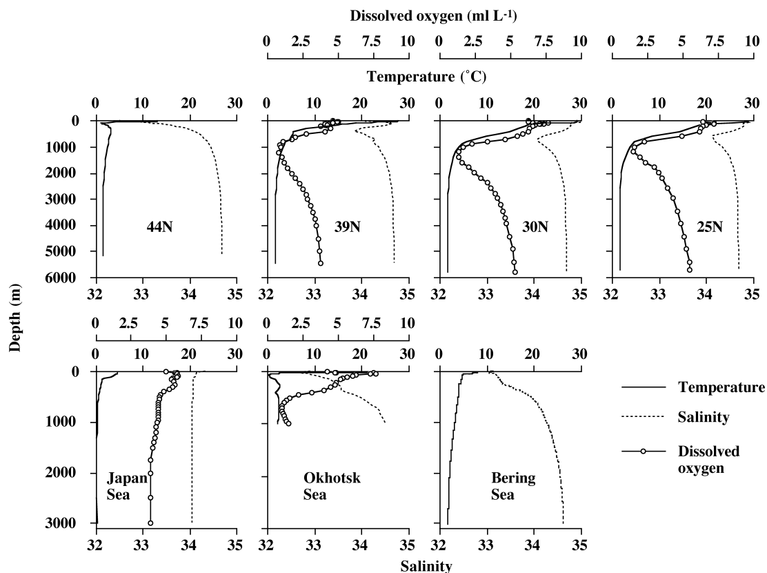
Fig. 2. Vertical profiles of temperature (°C), salinity, and dissolved oxygen ( ml\ L^{-1} ) in the western North Pacific Ocean (upper) and its adjacent seas (lower). Note that dissolved oxygen was not determined at St. 44N or in the Bering Sea. Depth scales are not the same between upper and lower panels.
