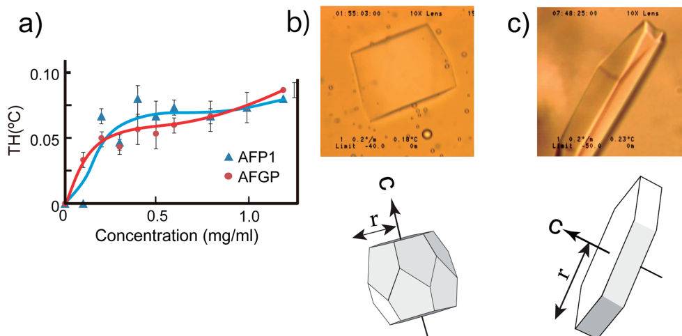
Figure 3 : Measurement of the TH and ice-shaping ability of the AFPs. (a) TH values plotted as a function of the concentration of AFPI (triangles) and AFGP (circles). For clarity, a smooth curve is drawn to fit each set of data. (b) Photomicrograph and illustration of an ice crystal created in a 0.6 mg/ml AFPI solution, showing a hexagonal trapezohedron shaped crystal with two flat basal planes. (c) Photomicrograph and illustration of an ice crystal created in a 0.6 mg/ml AFGP solution. This hexagonal plate is one of the derivatives of the hexagonal bipyramid as described in Griffith & Ewart (1995). The radius ( r ) in (b) is shorter than that in (c).
