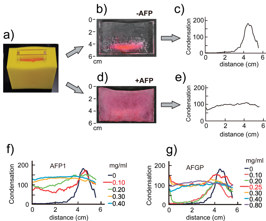
Figure 2 : Measurement of the FCI ability of AFPs. (a) An acrylic box (1×8×10 cm) containing the sample solution placed in a heat insulating material. One-directional freezing progresses from the opened top to bottom. (b) An ice block showing the condensed ink portion after overnight freezing of the sample without AFP. (c) The ink condensation plot created by a brightness tracing for (b). (d) An ice block showing a dispersion of the ink in the frozen sample containing AFPI. (e) The ink condensation plot created by a brightness tracing for (d). (f) Ink condensation profiles examined for 0–0.40 mg/ml solutions of AFP1. (g) Ink condensation profiles examined for 0–0.80 mg/ml solutions of AFGP.
