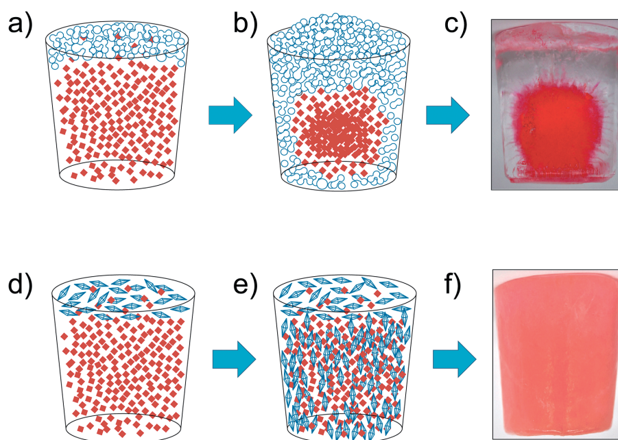
Figure 1 : Freeze concentration observed for an ordinary solution (a-c) and freeze-concentration inhibition (FCI) observed for the solutions containing AFPI (d-f). (a) Numerous seed ice crystals are created in the water solution at the moment it is frozen. The freezing is initiated near the top of the solution in this case. (b) Ice crystals bind to one another with time to form a multicrystalline state, which excludes the ink particles and concentrates them into an unfrozen portion of the vessel. (c) A snapshot of the entirely frozen ink solution without an AFP. The ink particles are trapped/concentrated in the middle of the ice block. (d) The seed ice crystals are created near the top of the water, while their growth and mutual binding are inhibited by AFPI. (e) The ice crystals assemble to form a slurry state, which cannot exclude the ink particles, leading to the formation of a frozen mixture of the ink and ice crystals. (f) A snapshot of the entirely frozen ink solution containing AFPI showing a uniformly colored ice block.
