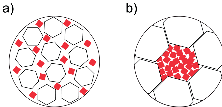
Figure 4 : A proposed mechanism for the FCI ability of the AFPs. (a) Illustration showing the spaces created between the growth-terminated ice crystals formed in the presence of AFPI, which should be capable of trapping the solute. AFPI creates thin ice crystals; thus, a smaller amount might be able to exhibit the FCI ability. (b) Illustration showing the creation of smaller spaces between the thick ice crystals, which tends to cause freeze concentration against the solute. Therefore, a larger amount of AFGP might be required to make the ice crystals smaller to provide the FCI ability.
