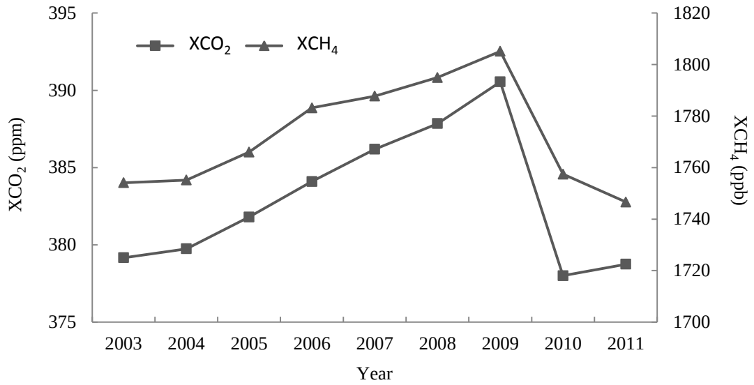
Fig. 5. \text{XCO}_2 and \text{XCH}_4 changes from 2003 to 2011, data from SCIAMACHY (2003-2009) and GOSAT (2010-2011) that covered the study area (regions that covered by the land cover image).
