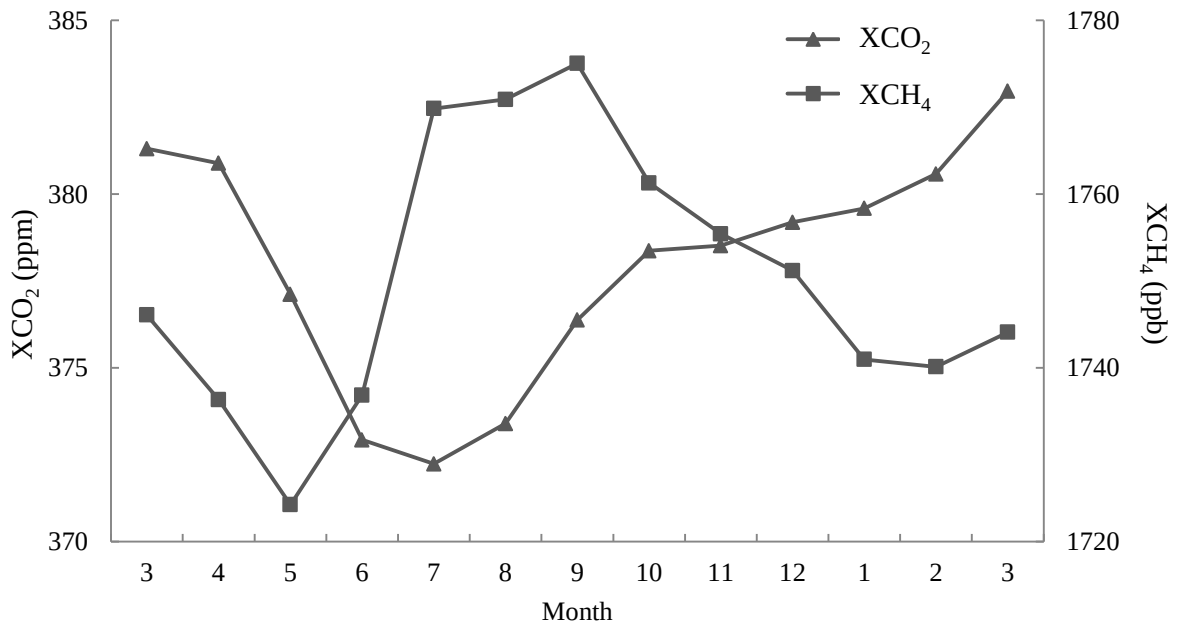
Fig. 6. The monthly \text{CO}_2 and \text{CH}_4 concentrations from March 2010 to March 2011.
