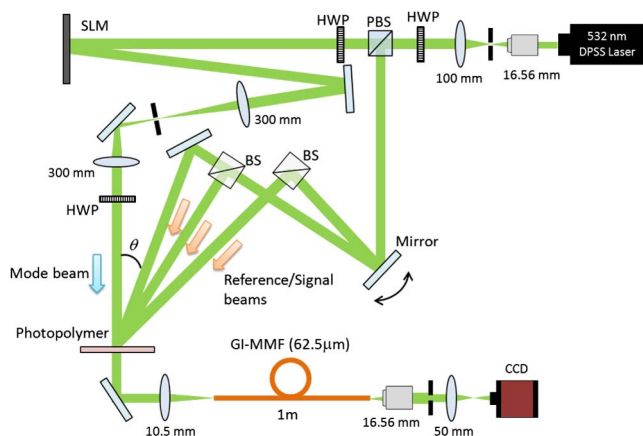
Fig. 2. (Color online) Experimental setup. HWP, half-wave plate; BS, beam splitter; PBS, polarizing beam splitter; SLM, spatial light modulator; GI-MMF, graded-index multimode fiber.
