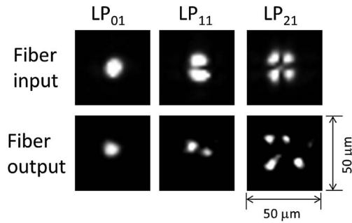
Fig. 4. Intensity profiles of the three modes at the fiber input and output.
