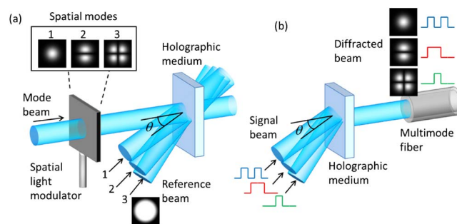
Fig. 1. (Color online) Concept of volume holographic mode multiplexer. (a) Recording process and (b) transmission process.
