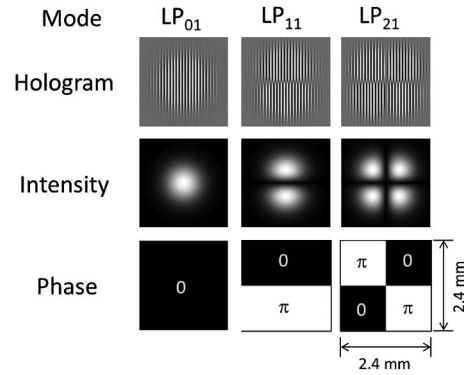
Fig. 3. Displayed hologram patterns on the SLM, and calculated mode fields of the intensity and the phase.
