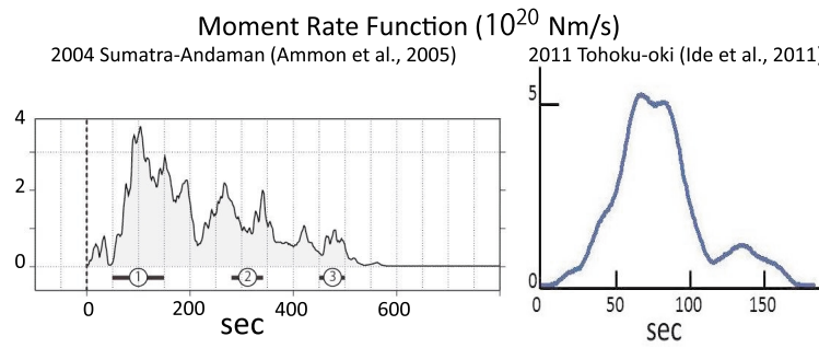
Fig. 4. Moment release time functions for the 2004 Sumatra-Andaman (Ammon et al. , 2005) and 2011 Tohoku-oki (Ide et al. , 2011) earthquakes.
