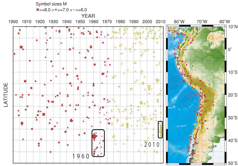
Fig. 2. Seismic activity along the Chilean subduction zone. We notice sparse seismicity prior to the 1960 and 2010 great earthquakes (seismic gap) and narrow seismically active area along the subduction zone. These are typical characteristics of ASSS. Epicenters relocated by Engdahl et al. (1998) are used from 1900 to 1972. From 1973 to July, 2011 USGS NEIC database 6 is analyzed. 6 http://earthquake.usgs.gov/earthquakes/eqarchives/epic/epic_global.php
