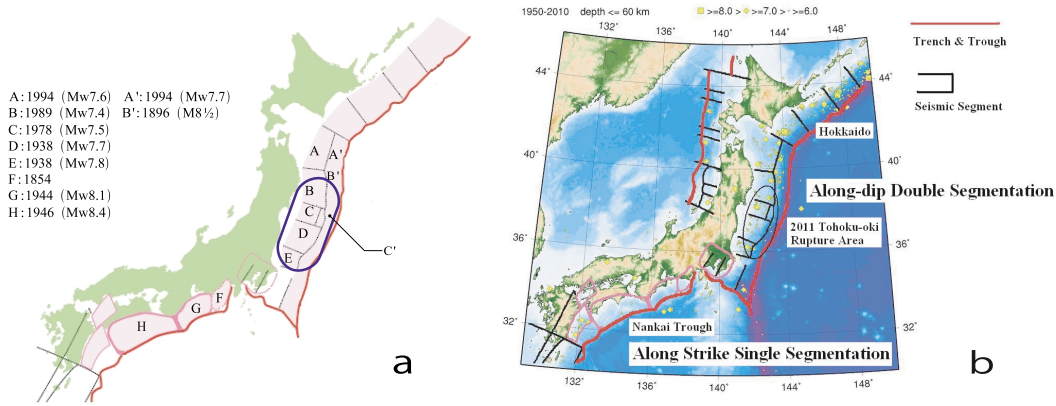
Fig. 1. Seismic activity in Japan and its vicinity. a : Seismic segmentation used in the official earthquake forecasting 5 of Evaluation of Major Subduction Zone Earthquakes by the Headquarters for Earthquake Research Promotion. The historical largest earthquake in each segment is indicated. b : Epicenters of earthquakes (yellow symbols classified by magnitude) from 1950 to 2010 with magnitudes by Japan Meteorological Agency equal to or larger than 6.0 and focal depths equal to or shallower than 60km. Trench and trough near Japan are illustrated by red curves. The 2011 Tohoku-oki megathrust earthquake ruptured the area circled by a solid ellipse, where along-dip double segmentation (ADDS, see text) is obvious. Along-strike single segmentation (ASSS) can be found in the Nankai Trough, where little recent seismic activity has been observed. Such regions are often called seismic gaps. 5 http://www.j-shis.bosai.go.jp/map/?lang=en (2010)
