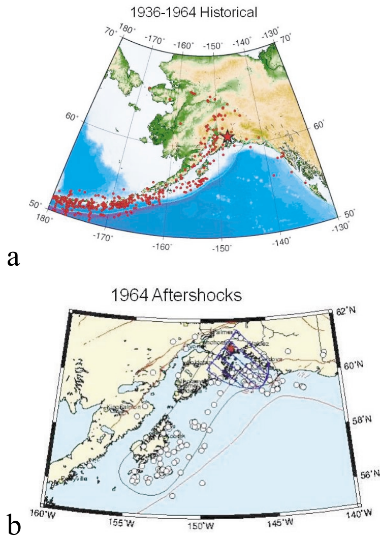
Fig. 3. Seismic activity prior to and after the 1964 Alaska earthquake (reproduced from Yomogida et al. , 2011). Historical earthquakes from 1936 to before the 1964 Alaska earthquake of which magnitudes are equal to or larger than 5.0 and focal depths equal to or shallower than 60km are plotted on the top. Aftershocks on the bottom are from Alaska Earthquake Information Center 7 , and the asperity from Ruff and Kanamori (1983) is indicated by shaded area. 7 http://www.aic.alaska.edu/quakes/Alaska_1964_earthquake.html
