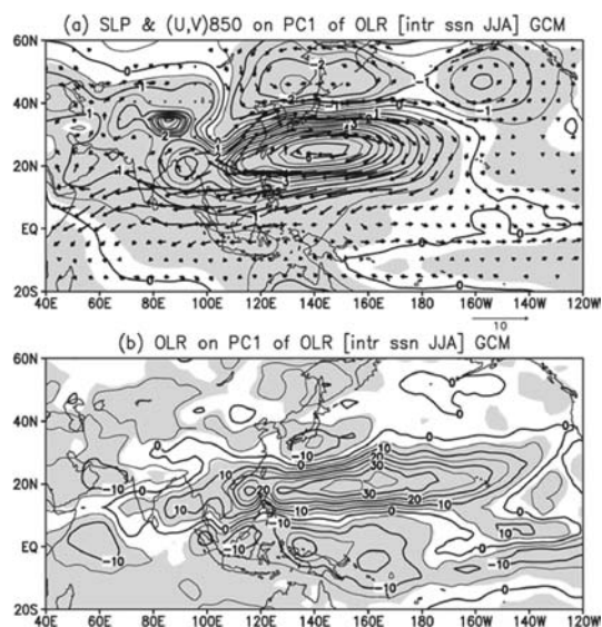
Fig. 7. (a) SLP (contour) and 850-hPa horizontal wind (vector) and (b) OLR regressed on the first principal component (PC) of intra-seasonal variation of OLR in 100^{\circ}\text{E} – 180^{\circ} and 10^{\circ}\text{S} – 50^{\circ}\text{N} for all ensemble members of the uncoupled GCM simulation. Contour interval is 0.5 hPa and wind vector reference is at the bottom right for (a). Shading denotes statistical significance at >5\% level.
