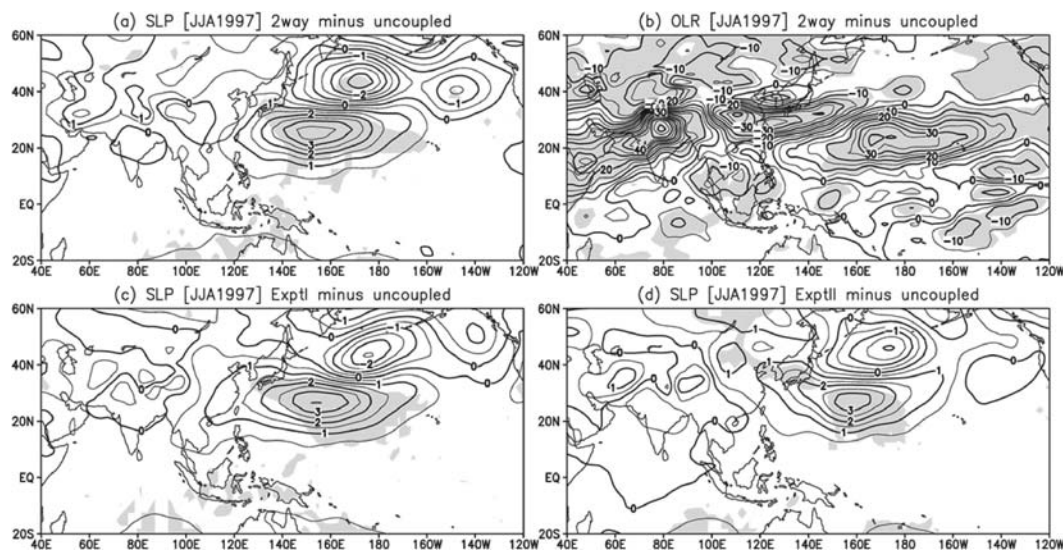
Fig. 6. SLP difference between two-way nesting GCM and uncoupled GCM in JJA 1997. Contour interval is 0.5 hPa with thick labels every 1 hPa. Shading denotes statistical significance at >5\% level. (b) Same as (a), but OLR with contour interval 5 \text{ W m}^{-2} . (c,d) Same as (a), but for (c) difference from Experiment I and (d) difference from Experiment II.
