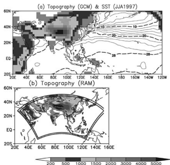
Fig. 3. (a) The surface height for the GCM (grayscale values as per the bottom reference) and sea surface temperatures (SSTs) averaged in June, July, and August (JJA) in 1997 (contour interval is 2 K and contours for 10, 20, and 28°C are indicated by thick dashed lines). (b) The surface height for the RAM (grayscale values) with the buffer zone between outer and inner thick lines.
