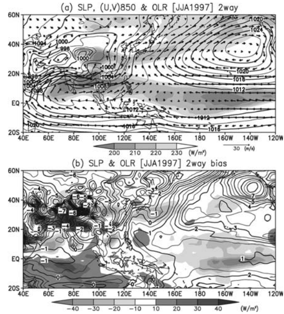
Fig. 5. Same as Figs. 4b,c, but for the two-way nesting GCM.
