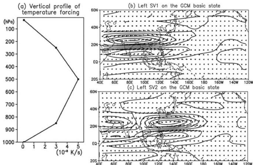
Fig. 9. (a) The vertical profile of the single-gridpoint temperature forcing in the singular vector (SV) calculation ( 10^{-5} \text{ K s}^{-1} ) based on the uncoupled GCM background. (b) Horizontal wind vector at 850 hPa and its horizontal rotation as components of the first SV estimated as the first empirical orthogonal functions (EOFs) for every response to single-gridpoint temperature forcing scattered over 60^{\circ}\text{E} – 180^{\circ} and 10^{\circ}\text{N} – 30^{\circ}\text{N} . (c) Same as (b), but for the second left SV.
