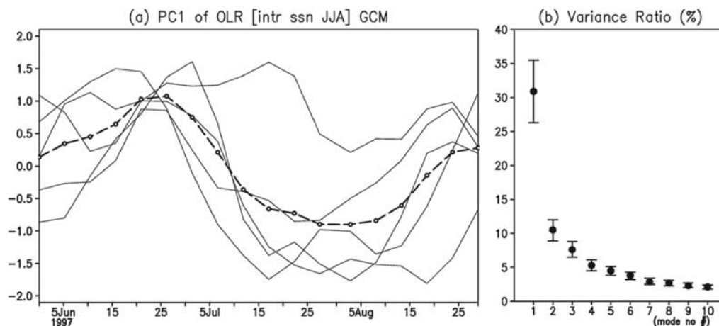
Fig. 8. The first PC of intra-seasonal variation of OLR in 100^{\circ}\text{E} – 180^{\circ} and 10^{\circ}\text{S} – 50^{\circ}\text{N} for JJA 1997 in the uncoupled GCM simulation. Thin solid lines denote normalized PCs for each ensemble run and the heavy dashed line denotes the ensemble average. (b) Variance ratio (%) of each PC mode to the total variance. The x -axis denotes the number of modes and error bars estimated following North et al. (1982).
