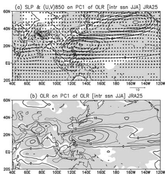
Fig. 1. (a) Sea-level-pressure (SLP; contour) and 850-hPa horizontal wind (vector) and (b) outgoing longwave radiation (OLR) regressed on the first principal component (PC) of intra-seasonal variation of OLR in 100°E–180° and 10°S–50°N for the JRA25 reanalysis data. Contour interval is 0.5 hPa and wind vector reference is at the bottom right for (a). Shading denotes statistical significance at >5% level.
