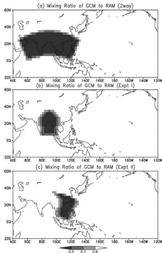
Fig. 2. The mixing ratio of the general circulation model (GCM) to the regional atmospheric model (RAM) common prognostic variables in the interactive mode experiments in INCL: (a) two-way standard experiment, (b) Experiment I, and (c) Experiment II. Gray shading as per the reference at the bottom.
