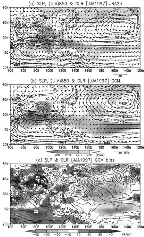
Fig. 4. SLP (contour), 850-hPa horizontal wind (vector), and OLR (shading) averaged in JJA 1997 (a) for the Japanese JRA25 reanalysis data and (b) for the ensemble-mean of the Atmospheric Model Inter-comparison Project (AMIP)-type simulation using an uncoupled GCM experiment. Contour interval is 2 hPa, thick labeled every 4 hPa; a vector reference is shown in the bottom right, and a shading reference is shown in the bottom of (b). (c) GCM bias for SLP and OLR, with contour interval 0.5 hPa and shadings as per the bottom reference.
