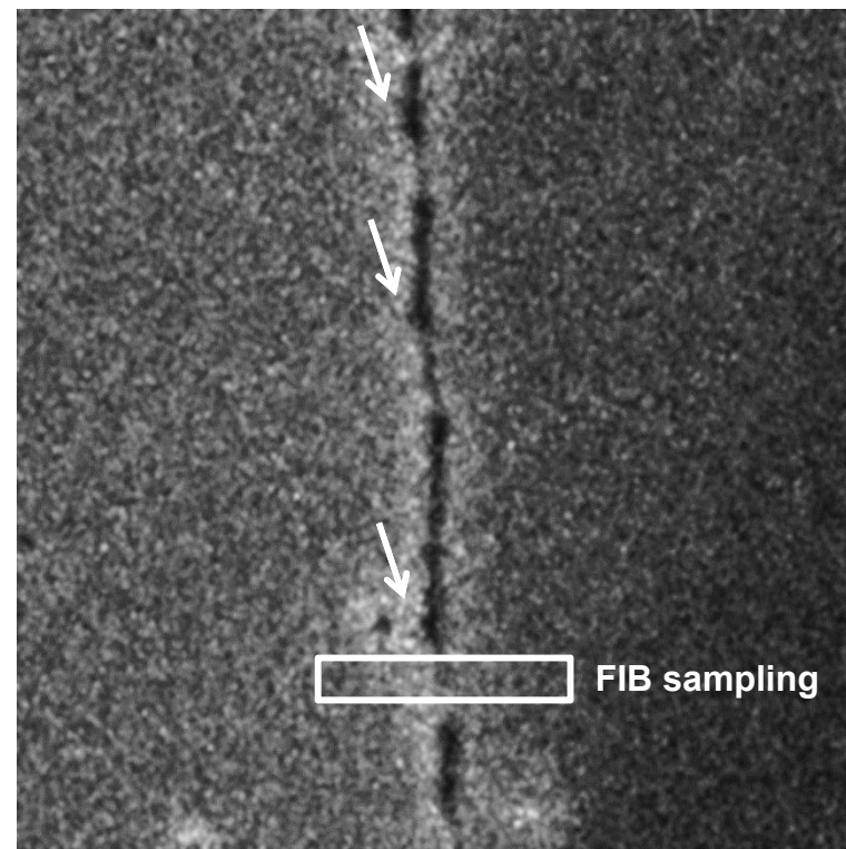
(b) \Sigma 9 CSLB (faceting)
