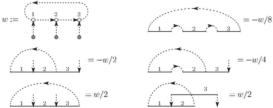
Fig. 5-6. All the chord diagrams in \mathcal{A}_3 (i-vertices are omitted).
