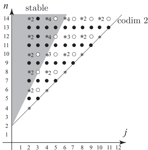
Fig. 3.1. • is a pair of dimension (j, n) where z_k \in \mathcal{A}_k \otimes \Omega_{DR}^{(n-j-2)k}(\text{Emb}(\mathbb{R}^j, \mathbb{R}^n)) is proved to be closed for all k \geq 2 , o is a pair (j, n) where z_k is proved to be closed for k \leq 4 , * is a pair where \hat{z}_k \in \mathcal{A}_k \otimes \Omega_{DR}^{(n-j-2)k}(\overline{\text{Emb}}(\mathbb{R}^j, \mathbb{R}^n)) is proved to be closed for all k \geq 2 , and *p indicates that \hat{z}_k descends to the closed form \bar{z}_k on \text{Emb}(\mathbb{R}^j, \mathbb{R}^n) for all k \geq p . We will show in Section 4 that z_k or \hat{z}_k in the range shown in this figure are nontrivial, provided that \mathcal{A}_k \neq 0 .
