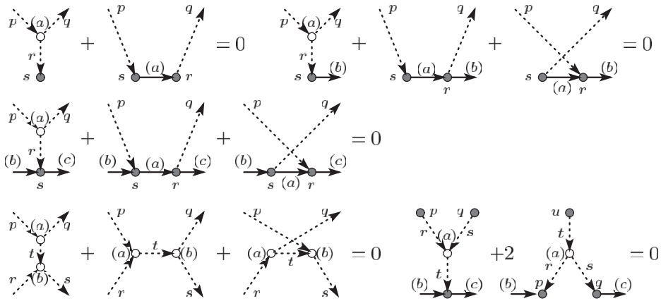
Fig. 2-2. ST, ST2, STU, IHX and Y relations, odd codimension case.
