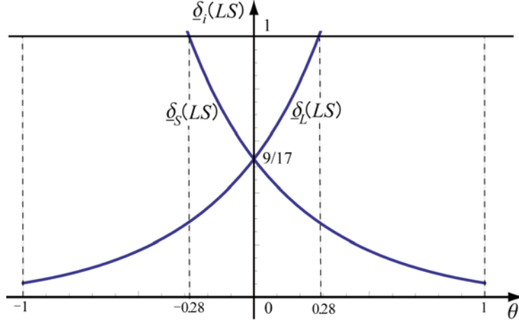
Figure 8: Loci of the minimum discount factors of countries L and S .
