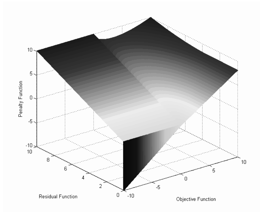
Figure 2: Shape of the extended oracle penalty function
