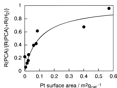
Figure 10. Selectivity of PCA production as a function of Pt surface area ( S_{\text{Pt}} ).
