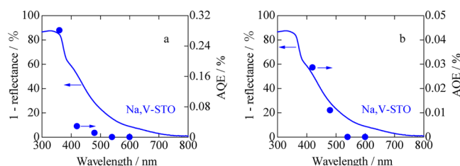
Figure 2. (a) Action spectrum for \text{O}_2 evolution from an aqueous \text{IO}_3^- solution over Ru/Na,V-STO accompanied by the UV–visible absorption spectrum of Na,V-STO. (b) Enlargement of (a).
