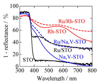
Figure 1. UV–visible absorption spectra of STO, Na,V-STO, Rh-STO, Ru/STO, Ru/Na,V-STO, and Ru/Rh-STO. After Ru deposition onto STO, Na,V-STO, and Rh-STO, increased absorption at a wider wavelength region ( >400 nm) was observed.
