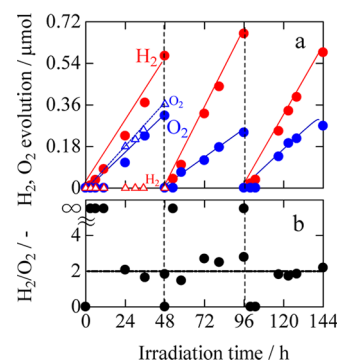
Figure 4. (a) Time courses of \text{H}_2 and \text{O}_2 (closed circles) evolution resulting from water splitting in the presence of Ru/Na,V-STO and Ru/Rh-STO photocatalysts irradiated with visible light ( >420 nm). The reaction was allowed to proceed for 144 h with evacuation every 48 h. In the first period up to 48 h, those of \text{H}_2 and \text{O}_2 (triangles) evolution in the presence of bare Na,V-STO and Rh-STO irradiated with visible light ( >420 nm) are plotted. (b) Ratio of evolved \text{H}_2 to \text{O}_2 in the presence of Ru/Na,V-STO and Ru/Rh-STO obtained from the data in (a). When only \text{H}_2 was detected in the initial period of the cycle, the ratio was indicated as \infty .
