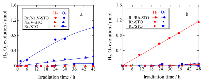
Figure 5. (a) Time courses of O 2 evolution resulting from half water splitting with the aid of IO 3 − sacrificial agent over Ru/Na,V-STO, bare Na,V-STO, and Ru/STO photocatalysts irradiated with visible light (>420 nm). In addition, plots of H 2 concentration were also included. However, H 2 concentrations in all cases were completely zero. (b) Time courses of H 2 evolution with the aid of I − over Ru/Rh-STO, bare Rh-STO, and Ru/STO photocatalysts irradiated with visible light (>420 nm). In addition, plots of O 2 concentration were also included. When either H 2 or O 2 gas was detectable, plots were indicated with a line. In contrast, either H 2 or O 2 gas was not observed at all; plots were indicated without a line.
