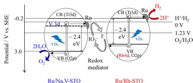
Figure 6. Schematic illustration of spontaneous H 2 and O 2 evolution by Ru/Na,V-STO and Ru/Rh-STO under irradiation with visible light in the presence of IO 3 − /I − redox mediator.
