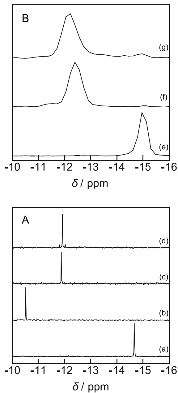
Fig. 2. (A) ^{31}\text{P} NMR spectra of (a) [\text{PW}_{12}\text{O}_{40}]^{3-} , (b) [\text{PW}_{11}\text{O}_{39}]^{7-} , (c) [\text{PW}_{11}\text{O}_{39}(\text{Sn-}n\text{-C}_4\text{H}_9)]^{4-} , and (d) [\text{PW}_{11}\text{O}_{39}(\text{Sn-OH})]^{4-} in 5:1 \text{H}_2\text{O}/\text{D}_2\text{O} (v/v) and (B) solid-state ^{31}\text{P} MAS NMR spectra of (e) Cs 3 -PW12 , (f) Cs 4 -PW11(Sn- n -Bu) , and (g) Cs 4 -PW11(Sn-OH) .
