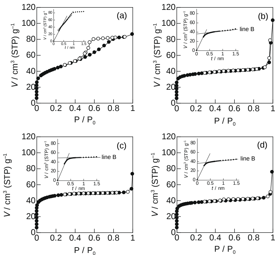
Fig. 6. Adsorption-desorption isotherms of N_2 at 77 K for (a) \text{Cs}_3\text{-PW12} , (b) \text{Cs}_4\text{-SiW12} , (c) \text{Cs}_4\text{-PW11(Sn-}n\text{-Bu)} , and (d) \text{Cs}_4\text{-PW11(Sn-OH)} . Insets are t -plots calculated from corresponding N_2 adsorption isotherms.
