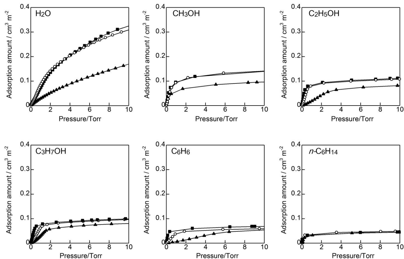
Fig. 9. Adsorption isotherms of water, methanol, ethanol, 1-propanol, benzene, and n -hexane on microporous Cs salts. ( \circ ) \text{Cs}_4\text{-SiW}_{12} , ( \blacktriangle ) \text{Cs}_4\text{-PW}_{11}(\text{Sn-}n\text{-Bu}) , and ( \blacksquare ) \text{Cs}_4\text{-PW}_{11}(\text{Sn-OH}) .
