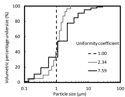
Fig.3. Fictitious adsorbent particle size distributions with the same D_{40} (1.0 μm) for BPKM-SAM simulations.
