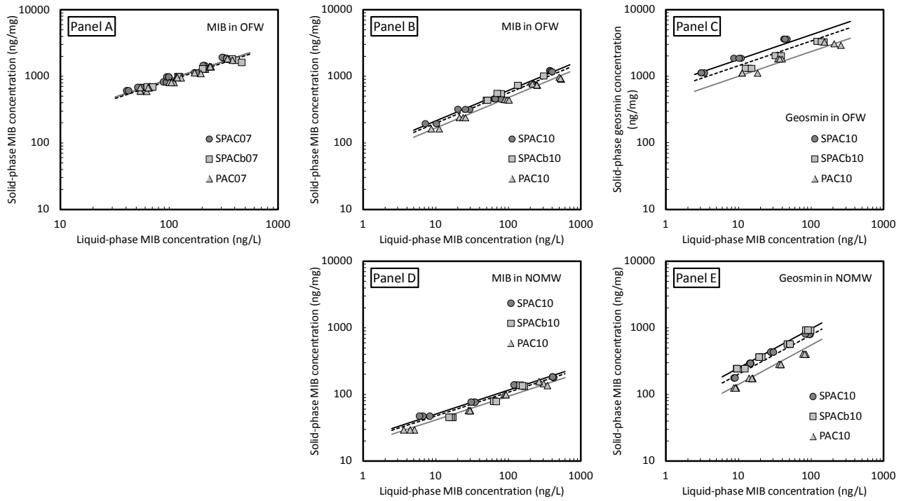
Fig. 1. Adsorption isotherms for MIB (Panels A, B, and D) and geosmin (Panels C and E). Experimental data are shown as points, and SAM fits to the data are shown as lines. The SAM fit parameters are as follows: Panel A — K_0 : 3.1 \text{ (mg/g)/(ng/L)}^{1/n} , \delta : 38.6, 1/n : 0.54 Panel B — K_0 : 1.8 \text{ (mg/g)/(ng/L)}^{1/n} , \delta : 9.1, 1/n : 0.46 Panel C — K_0 : 10.7 \text{ (mg/g)/(ng/L)}^{1/n} , \delta : 3.0, 1/n : 0.37 Panel D — K_0 : 0.3 \text{ (mg/g)/(ng/L)}^{1/n} , \delta : 11.0, 1/n : 0.36 Panel E — K_0 : 4.1 \text{ (mg/g)/(ng/L)}^{1/n} , \delta : 3.2, 1/n : 0.59.
