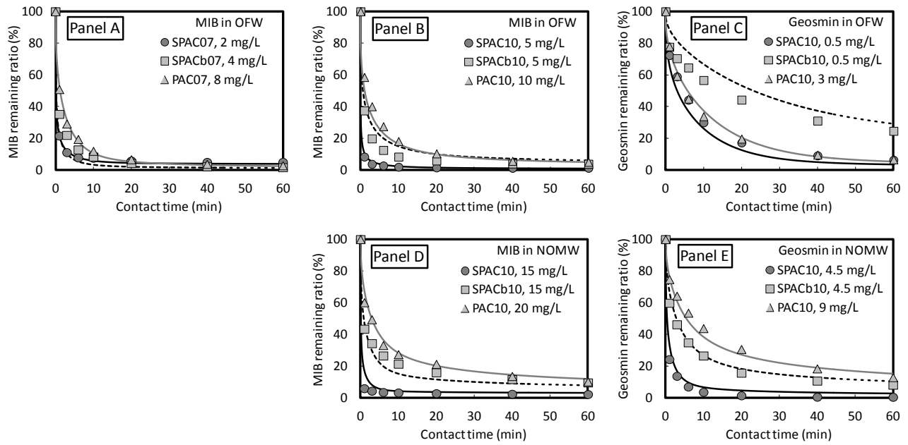
Fig. 2. Adsorption kinetics for MIB (Panels A, B, and D) and geosmin (Panels C and E). Experimental data are shown as points, and BPKM-SAM simulations are shown as lines. Initial MIB and geosmin concentrations are \sim 1 \mu\text{g/L} . The BPKM-SAM parameters are as follows: Panel A — D_p : 1.7 \times 10^{-7} \text{ cm}^2/\text{s} , k_s : 8.7 \times 10^{-4} \text{ s}^{-1} , \phi : 0.57 Panel B — D_p : 3.1 \times 10^{-7} \text{ cm}^2/\text{s} , k_s : 3.9 \times 10^{-4} \text{ s}^{-1} , \phi : 0.73 Panel C — D_p : 2.1 \times 10^{-7} \text{ cm}^2/\text{s} , k_s : 3.8 \times 10^{-4} \text{ s}^{-1} , \phi : 0.29 Panel D — D_p : 3.0 \times 10^{-7} \text{ cm}^2/\text{s} , k_s : 2.1 \times 10^{-3} \text{ s}^{-1} , \phi : 0.55 Panel E — D_p : 0.44 \times 10^{-7} \text{ cm}^2/\text{s} , k_s : 1.5 \times 10^{-3} \text{ s}^{-1} , \phi : 0.53.
