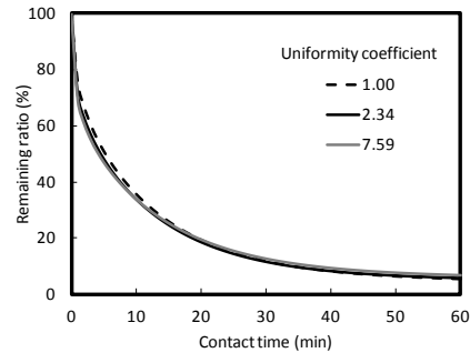
Fig. 4. Effect of particle size distribution on adsorption kinetics of geosmin: BKAM-SAM simulations ( D_{40} = 1.0 \mu\text{m} , activated carbon dose = 0.5 \text{ mg/L} , initial geosmin concentration: 1000 \text{ ng/L} , NOM water, D_S: 2.1 \times 10^{-7} \text{ cm}^2/\text{s} , k_S: 3.8 \times 10^{-4} \text{ s}^{-1} , \phi: 0.29 ).
