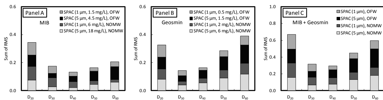
Fig. 5. Sums of root mean square (RMS) values to select the best characteristic size that represents a group of adsorbent particles with the same size distribution (Initial MIB or geosmin concentration is 1000 ng/L).
