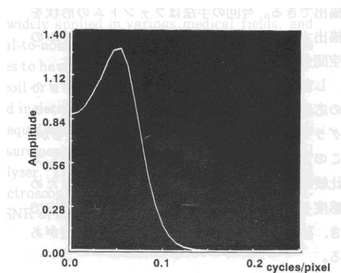
Figure 7 Spatial frequency characteristics of filter used for restoration shown in Figure 6. Parameter m was 5.0 and parameter c was 1.5 \times 10^{-1} .
