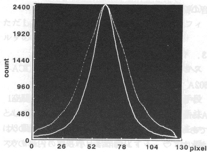
Figure 3 Point spread functions. Solid and dotted lines represent source-camera distances of 0 and 2.3 cm, respectively.
