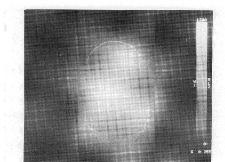
Figure 2 Uncollimated image at phantom-camera distance of 0 cm. White line indicates outline of actual phantom.
