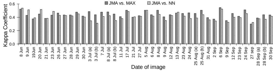
Figure 1. Comparison of K_{\text{hat}} values between JMA vs. MAX and JMA vs. NN for selected images during JJAS 2010.
