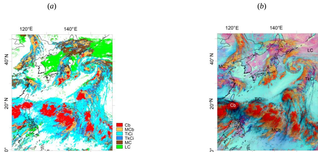
Figure 3. (a) Cloud-type classification result obtained using 2D-THR algorithm and (b) its corresponding night-time microphysical colour composite for 2 August 2009 at 02:30 UTC.
