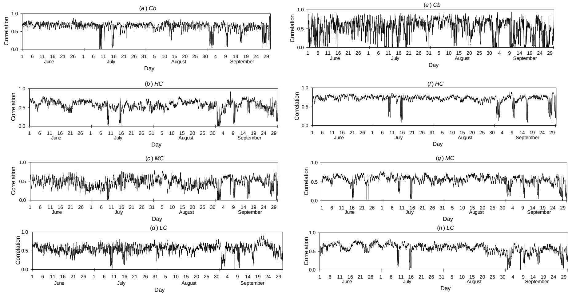
Figure 5. Hourly variation in the spatial correlation of Cb ((a) and (e)), HC ((b) and (f)), MC ((c) and (g)) and LC ((d) and (h)) percentage between 2D-THR and JMA cloud classification for tropical region ((a)–(d)) and subtropical region ((e)–(h)) during June, July, August and September 2009.
