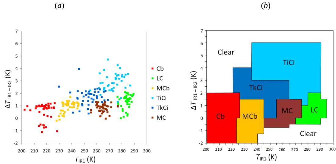
Figure 2. (a) A scatter plot of mean centre of each cloud type derived from MAX classification results; (b) 2D-THR for cloud-type classification by using T_{\text{IR1}} and \Delta T_{\text{IR1-IR2}} of MTSAT 1R.
