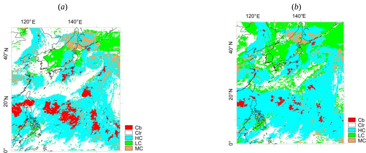
Figure 4. Inter-comparison of the reclassified cloud type classification between (a) 2D-THR cloud type classification result and (b) the JMA product for 2 August 2009 02:30 UTC. 2D-THR is resampled into the same spatial resolution as JMA.
