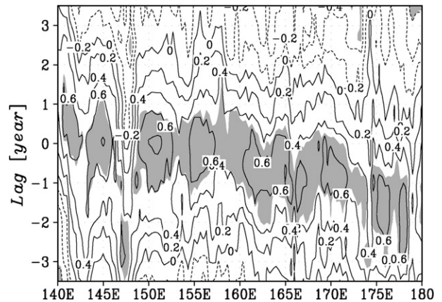
FIG. 9. Lag correlations of PC1 with the monthly-mean latitude of the KE jet: contour interval 0.1; shading indicates the regions where the correlations are significant at the 95% confidence level. Negative lag means that PC1 lags. Before calculating the correlations, a 9-month running mean filter is applied to the jet latitude data.
