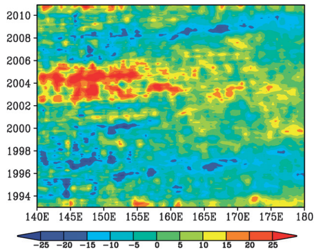
FIG. 13. Monthly mean jet absolute speed anomalies along the KE jet axis ( \text{cm s}^{-1} ): jet speed data are smoothed by a 9-month running mean filter.
