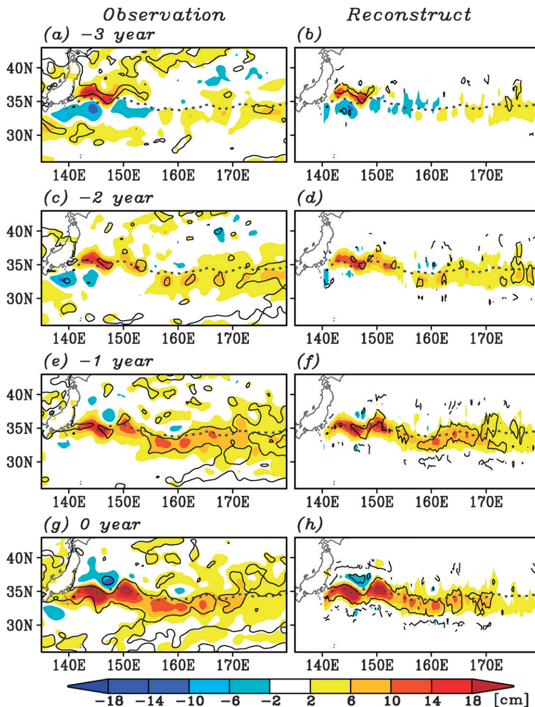
FIG. 7. Lag regressions of SLAs (left) of the satellite observation and (right) by the reconstruction (Eq. 1) onto PC1 for lag year (a),(b) -3 ; (c),(d) -2 ; (e),(f) -1 ; (g),(h) 0 ; negative lag means that PC1 lags SLAs. The SLA data are smoothed by a 9-month running mean filter. The black solid contour indicates the regions where the corresponding correlations are significant at the 95% confidence level. The gray dotted line denotes the climatological position of the KE jet. In the right column, statistical significance of the correlations is not drawn for the regions where absolute values of the corresponding regressions are less than 0.5 cm.
