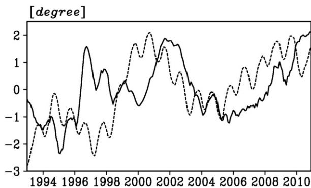
FIG. 15. Observed latitude anomalies of the KE jet averaged over 175^{\circ}\text{E} – 180^{\circ} (solid line) and estimated from SLAs integrated over 30^{\circ} – 40^{\circ}\text{N} and averaged over 150^{\circ} – 170^{\circ}\text{W} (dashed line). The two time series are smoothed by a 9-month running mean filter.
