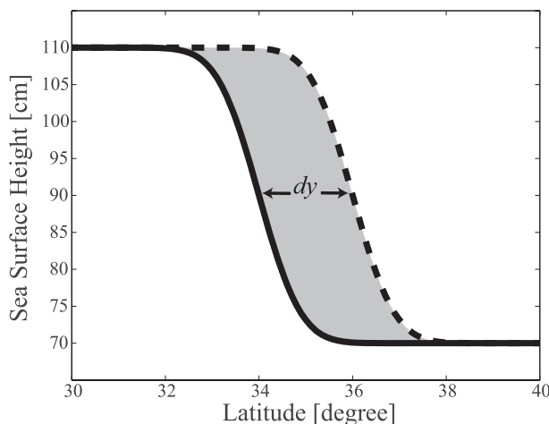
FIG. 11. Schematic diagram illustrating the reconstruction of sea level variability using Eq. (1). The solid line denotes the climatological sea surface height of the jet. Its northward displacement dy , shown by the dashed line, induces SLAs indicated by the gray shading.
