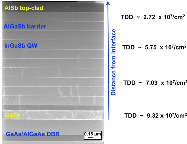
Figure 15: STEM image of lattice mismatched III-Sb VECSEL on GaAs/AlGaAs showing the source of the threading dislocations at the IMF array and subsequent reduction in the density as a function of distance from the mismatched interface.
