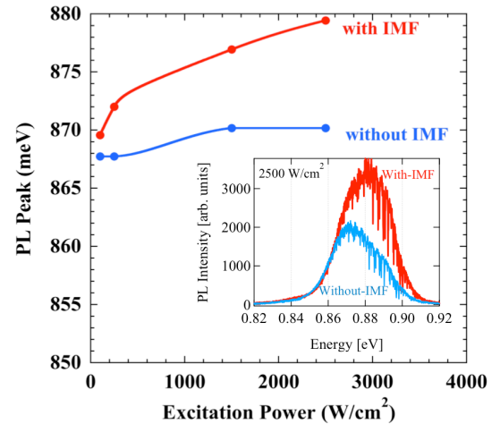
Figure (17) PL peak shift with the excitation power. Clear blue shift is observed with QW with IMF. Inset is the PL spectra measured at the excitation power of 2500 W/cm 2 on QWs grown with IMF and without IMF.
