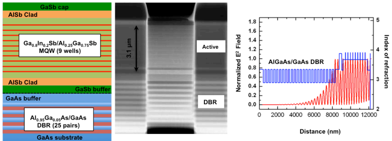
Figure 2: Schematic, cross-section TEM image and plot of refractive index and E-field for lattice-mismatched 2μm III-Sb VECSEL grown on GaAs/AlGaAs DBR.
