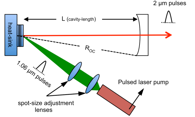
Figure 10: Schematic for optically pumped VECSEL operated in pulsed mode.
