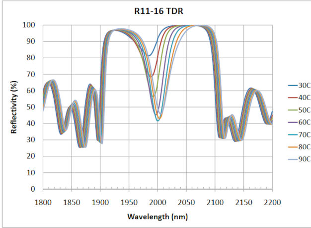
Figure 9: Temperature dependent reflectivity spectra from a VECSEL on GaAs/AlGaAs DBR.
