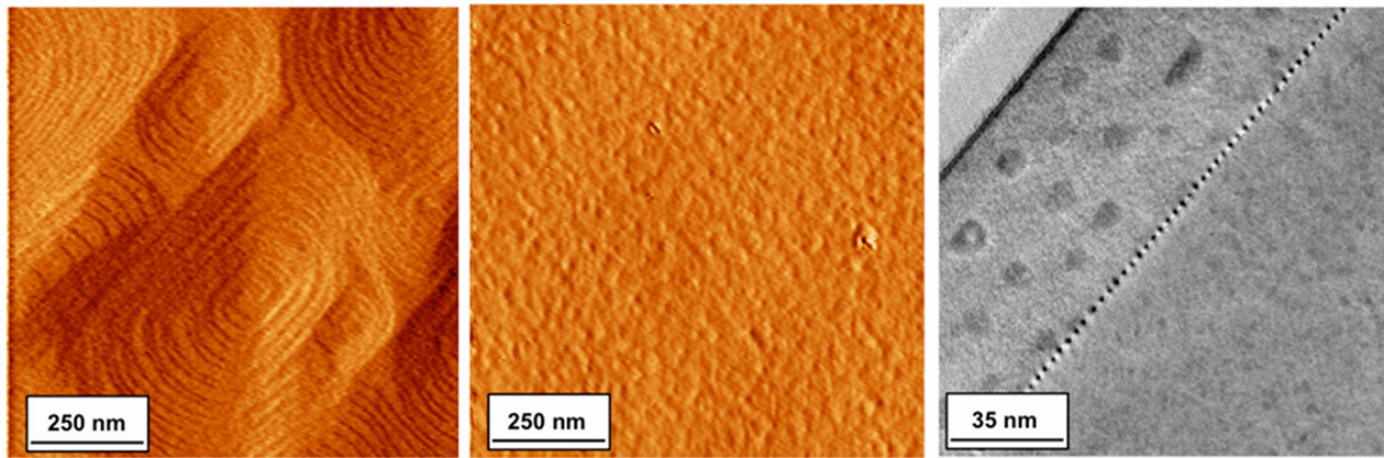
Figure 3: (a) Atomic force micrograph of GaSb on GaAs without the formation of the IMF array. (b) Atomic force micrograph of GaSb on GaAs with an optimized IMF array at the GaSb/GaAs interface. (c) cross-section TEM image of GaSb grown on GaAs with a periodic IMF array at the interface.
