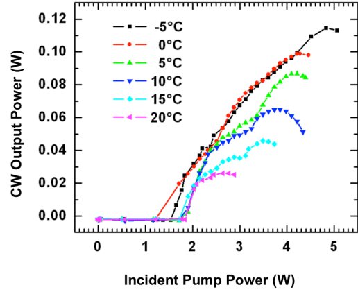
Figure 13: Output-power Vs Pump power for the CW III-Sb VECSEL on GaAs substrate.
