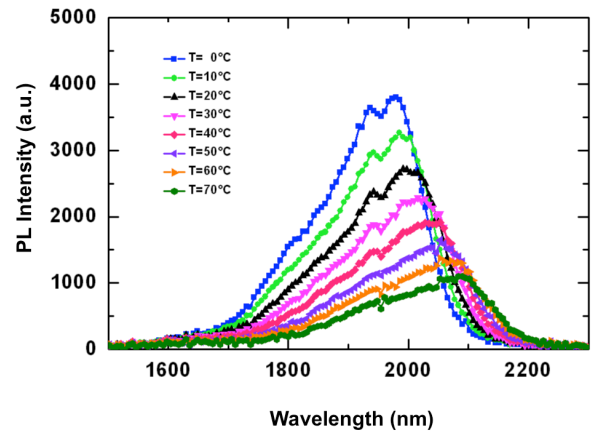
Figure 7: Edge PL spectra from a VECSEL sample.
