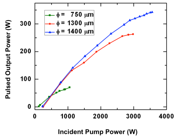
Figure 11: Peak output-power Vs peak pump power for the pulsed III-Sb VECSEL on GaAs substrate.
