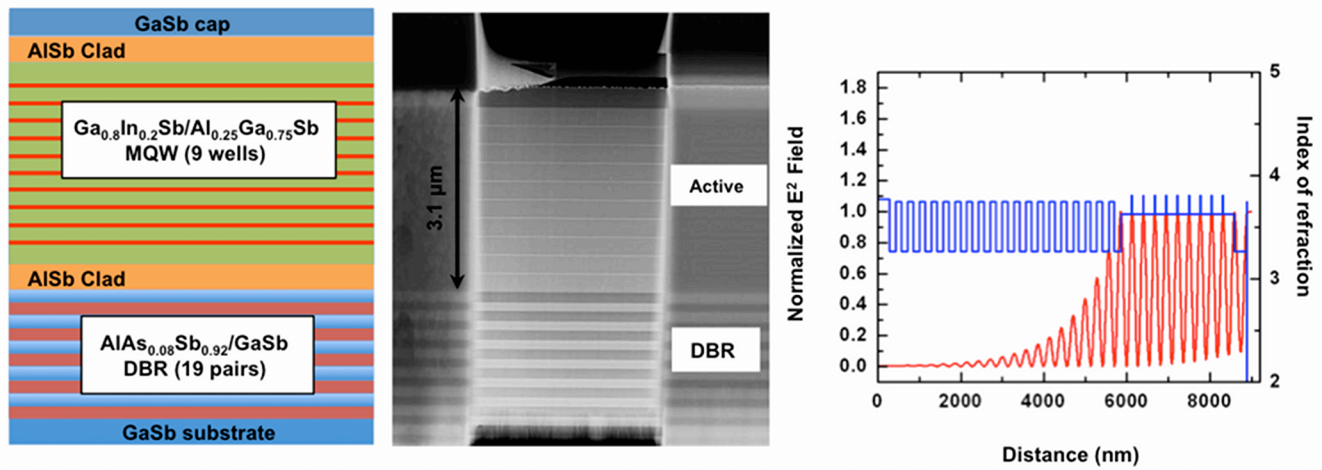
Figure 1: Schematic, cross-section TEM image and plot of refractive index and E-field for lattice-matched 2μm III-Sb VECSEL grown on GaSb/AlAsSb DBR.
