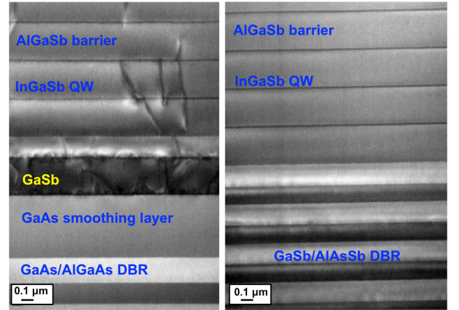
Figure 14: Transmission electron microscopy comparison of lattice mismatched III-Sb VECSEL on GaAs/AlGaAs to lattice matched VECSEL on GaSb/AlAsSb. Figure (a) shows the lattice mismatched structure with extensive threading dislocations in the active region and (b) shows the complete absence of threading dislocations in the lattice matched structure.
