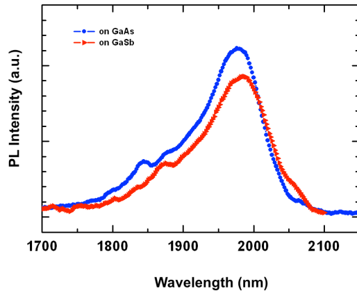
Figure (4) PL of a structure with 11 nm thick \text{Ga}_{0.75}\text{In}_{0.25}\text{Sb} quantum wells, grown on a GaAs substrate (blue), and grown on a GaSb (red).
