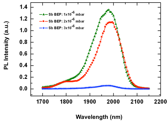
Figure (6) Influence of the Sb flux, measured as beam equivalent pressure (BEP) on the PL of a VECSEL active region with 9 quantum wells (grown on GaAs).
