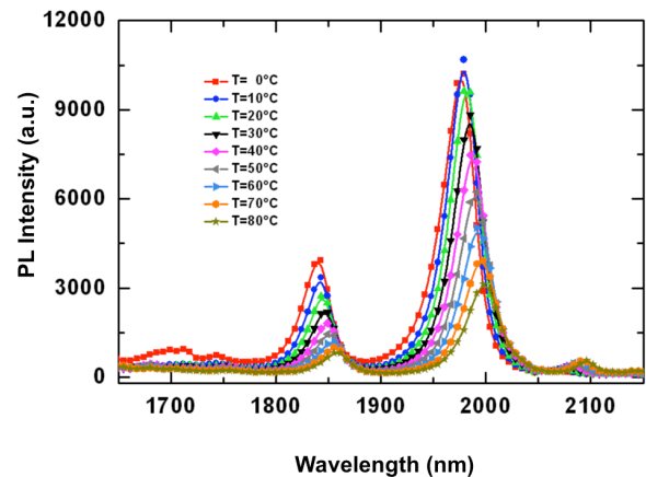
Figure 8: Surface PL spectra from a VECSEL sample.
