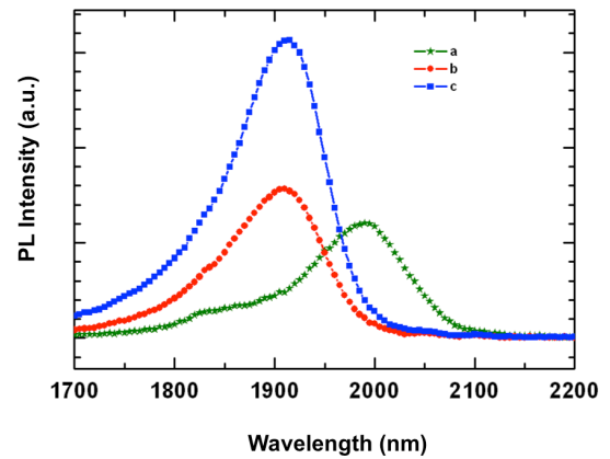
Figure (5) PL of a structure with 10 nm thick \text{Ga}_{0.72}\text{In}_{0.28}\text{Sb} quantum wells, grown at 475^\circ\text{C} (a), and at near 490^\circ\text{C} (b). For comparison the emission wavelength of b can also be achieved by a structure with 12 nm thick \text{Ga}_{0.8}\text{In}_{0.2}\text{Sb} well, grown at 475^\circ\text{C} (c).
