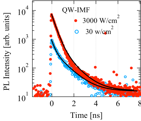
Figure (16) Transient PL decay measured on QWs grown with IMF with the average excitation powers of 30 W/cm 2 and 3000 W/cm 2 .
