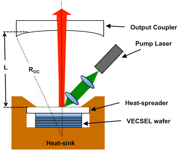
Figure 12: Schematic for optically pumped VECSEL operated in CW mode.
