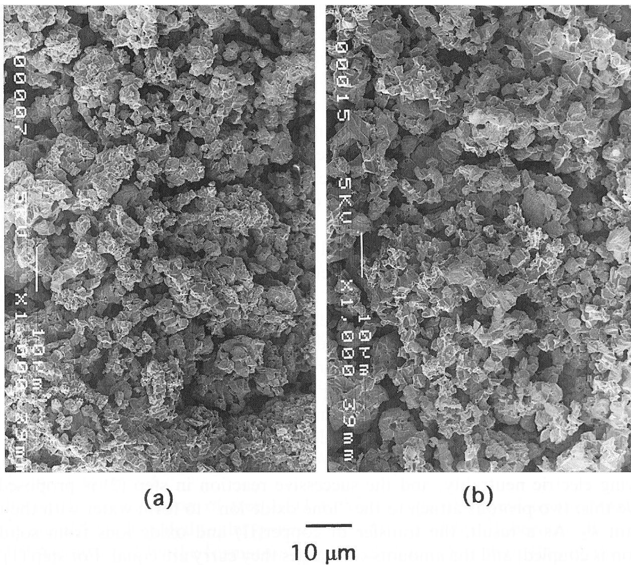
Fig. 4. Electron micrographs of CuO specimen. (a) Before and (b) after dissolution experiment.
