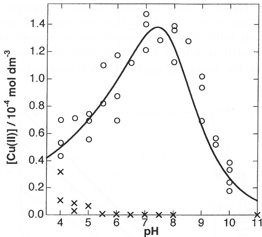
Fig. 2. Relationship between dissolved Cu concentration [\text{Cu(II)}] and pH in 3 \times 10^{-3} \text{ mol dm}^{-3} EDTA solutions at 80^\circ\text{C} after 5 h. With EDTA (O), without EDTA (x); curve calculated with Eq. (14).
