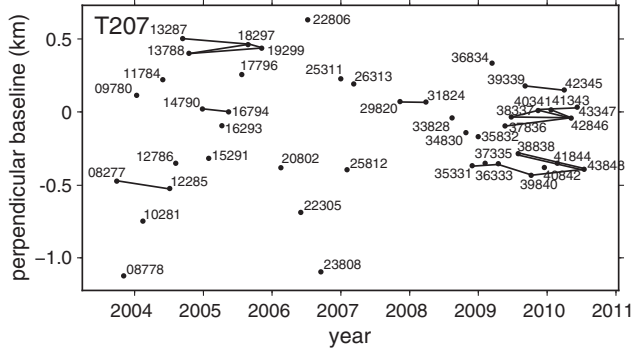
Figure A2. Envisat SAR data from the descending track 207. The dots and lines have the same meaning as in Figure A1.
