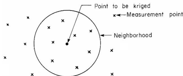
Figure A. 13 Kriging with a moving neighborhood (de Marsily 1986)
