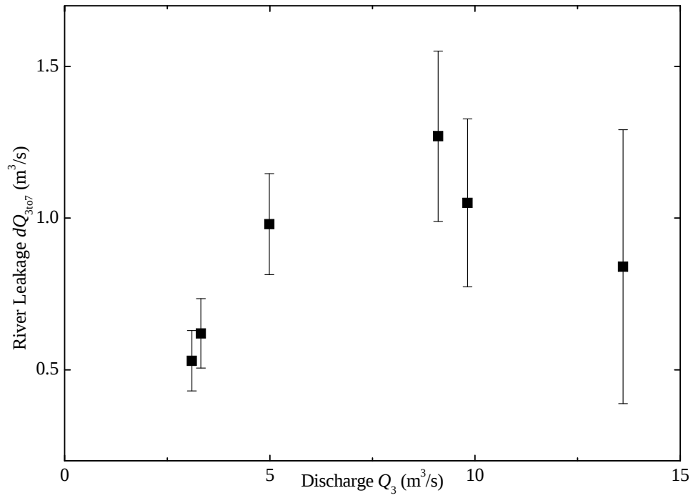
Figure 3.9 Relation between river discharge and leakage. Q_3 and dQ_{3to7} are discharge at St.3 and leakage between St.3 and St.7. Error bars are the estimated standard deviation of leakage.
