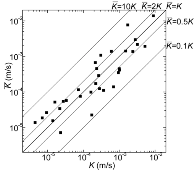
Figure 4.9 Comparison in double logarithmic scale between hydraulic conductivities measured by slug test ( K (m/s)) and estimated by Eq. (4.9) ( \bar{K} (m/s)). Here, R^2 = 0.80
