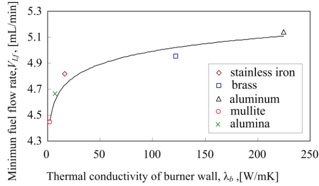
Fig. 5 Relationship between minimum fuel flow rate and thermal conductivity of burner wall ( T_{air} = 293 K)
