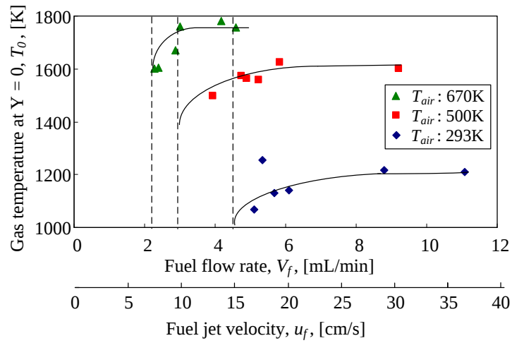
Fig. 11 Variation gas temperature at Y = 0 against the imposed fuel flow rate under three preheated air temperature conditions ( T_{air} = 293\text{ K} , 500\text{ K} , 670\text{ K} )
