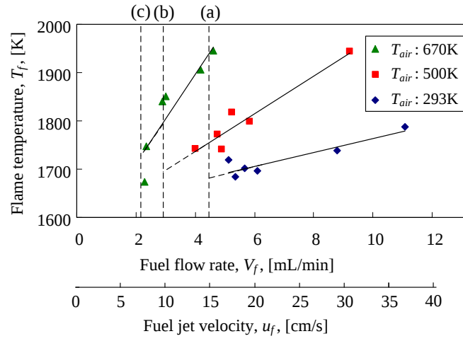
Fig. 10 Variation of maximum flame temperature against the imposed fuel flow rate under three preheated air temperature conditions ( T_{air} = 293\text{ K} , 500\text{ K} , 670\text{ K} )
