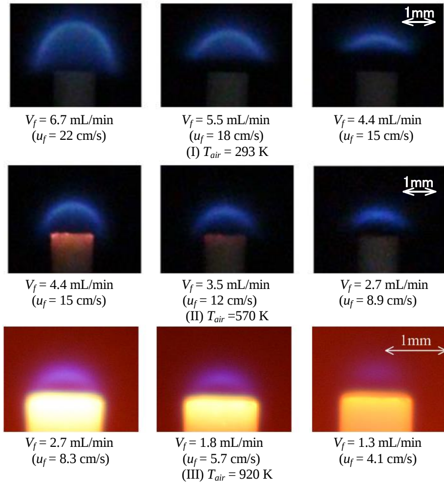
Fig. 4 Direct photograph of the microflames under three preheated air temperature conditions ( T_{air} = 293 K, 570 K, 920 K) and various fuel flow rates (fuel jet velocity at standard state is also shown).
