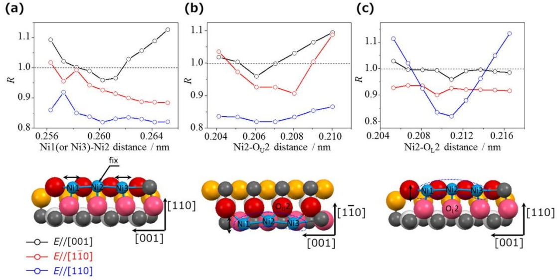
Figure 7. R value as a function of the Ni coordinate. R value calculated for the E//[001] direction, E//[\bar{1}\bar{1}0] direction and E//[110] direction are shown in black, red, and blue, respectively. (a) Ni1 and Ni3 coordinates were symmetrically changed along the [001] direction. (b) Ni trimer cluster was moved along the [\bar{1}\bar{1}0] direction while holding the three Ni relative positions constant (c). Ni trimer cluster was moved along the [110] direction while holding the three Ni relative positions constant.
