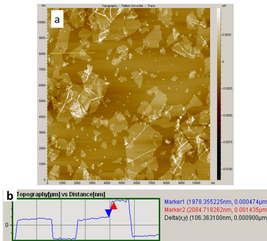
Fig. 3. Fully exfoliated GO sheets on freshly mica (a) and a topographic image of sheets (b).
