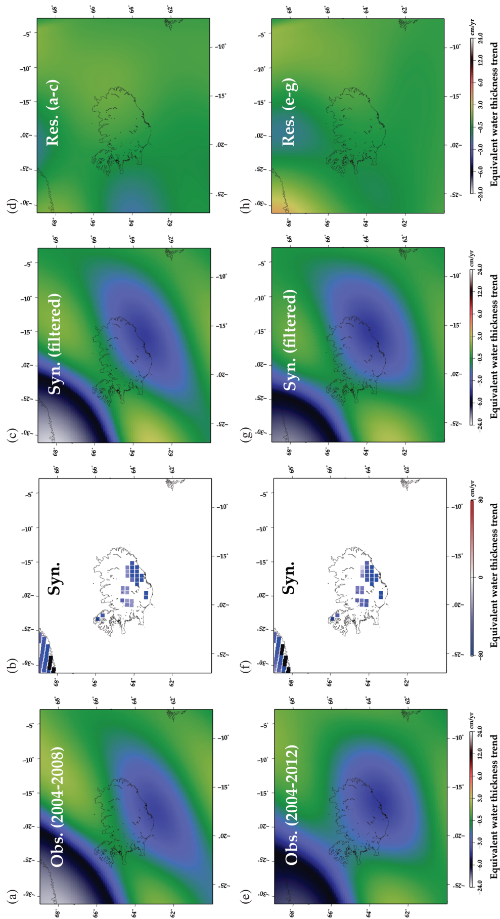
Fig. 3. Distributions of the EWT linear trends in Iceland. (a) - (d) are for the period 2004.02 - 2012.01. (e) and (f) are the linear trends observed by GRACE, (b) and (f) are synthesized linear trend obtained using point-mass modeling, (c) and (g) are synthesized linear trend after applying the same filter as GRACE, and (d) and (h) are the residual between the observed (a) (e), and the synthesized (c) (g), respectively.
