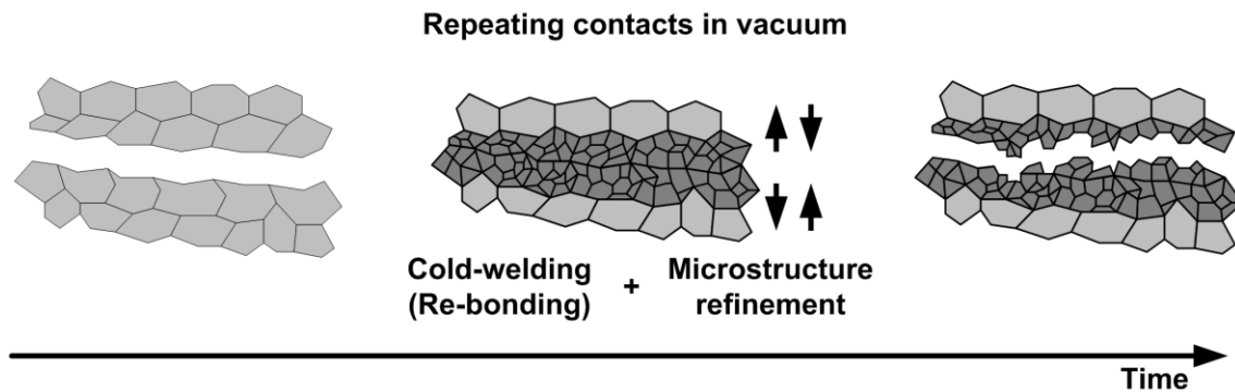
Fig. 9. Model of the formation of a granular region based on the cold-welding (re-bonding).
