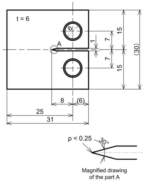
Fig. 3. Specimen configuration (CT).
