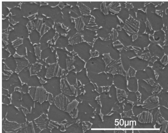
Fig. 2. Microstructure of Ti-6Al-4V.
