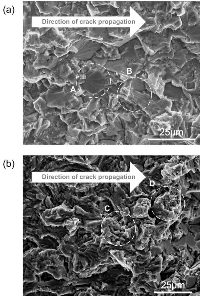
Fig. 6. Fracture surfaces of the crack propagation tests, (a) Air ( K = \Delta 7 \text{ MPa}\sqrt{\text{m}} ) and (b) HV ( 2.7 \times 10^{-5} \text{ Pa} , \Delta K = 8 \text{ MPa}\sqrt{\text{m}} ).
