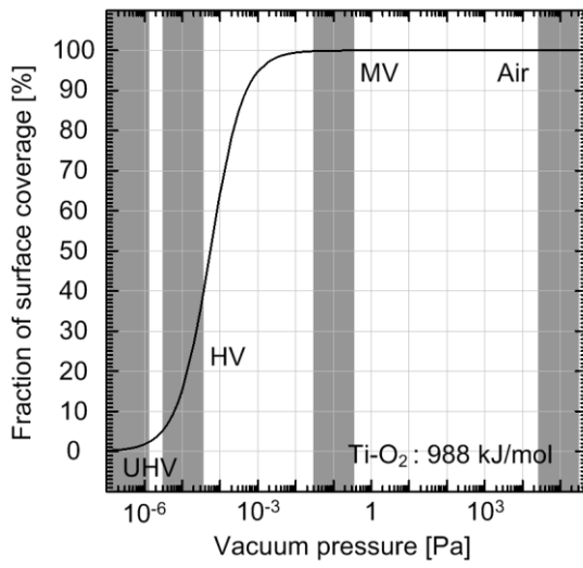
Fig. 8. Relation between the fraction of surface coverage and vacuum pressure.
