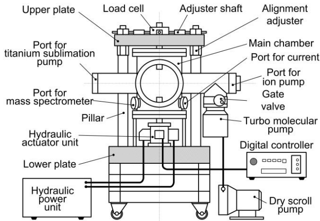
Fig. 4. Ultra high vacuum fatigue testing machine.
