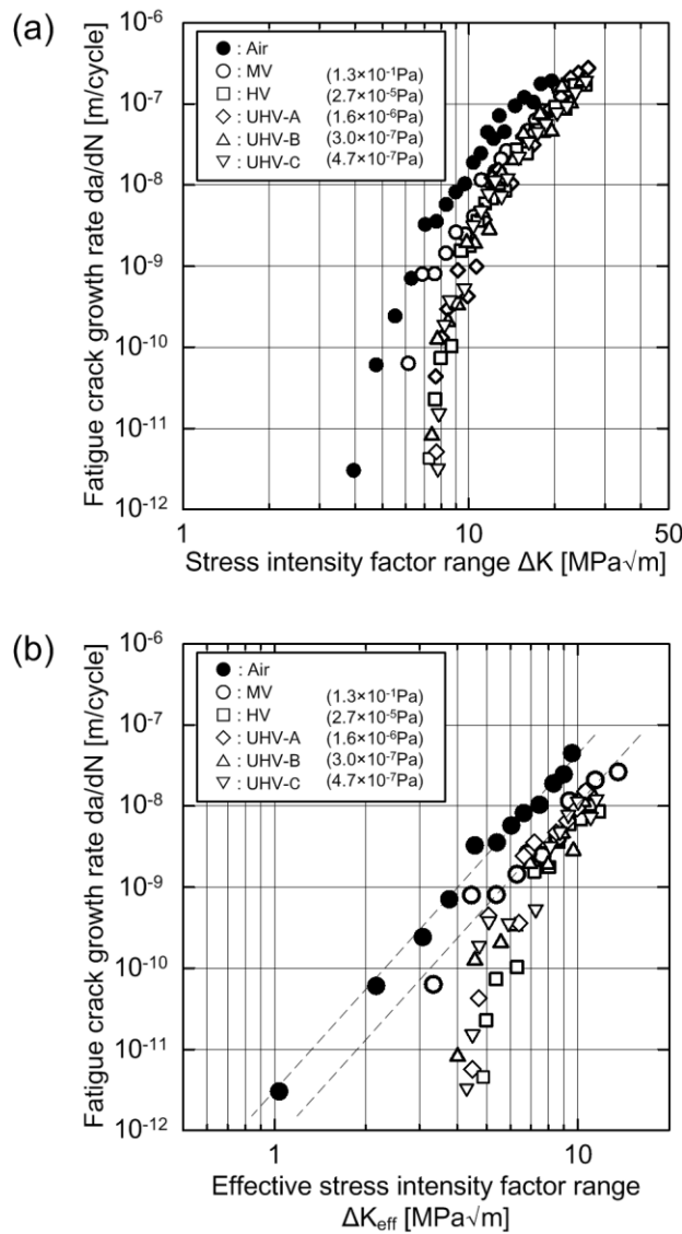
Fig. 5. Results of fatigue crack propagation tests, (a) da/dN - \Delta K and (b) da/dN - \Delta K_{\text{eff}} .
