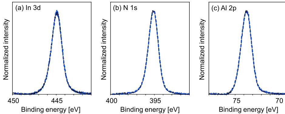
Fig. 3 (a) In 3d, (b) N 1s, and (c) Al 2p spectra. Solid lines indicate the spectra obtained after air exposure for 1 h after 1 min of HF treatment, while broken lines indicate the spectra obtained immediately after the HF treatment.
