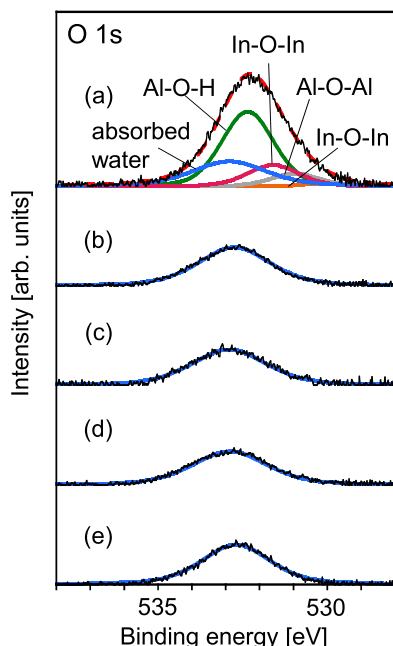
Fig. 2 O1s spectra obtained for (a) untreated sample and samples treated with (b) HF for 1 min, (c) 1-h air exposure after 1-min HF treatment, (d) BHF for 5 min, and (e) 1-h air exposure after 5-min BHF treatment.
