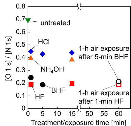
Fig. 1 [O 1s]/[N 1s] vs treatment time or exposure time.
