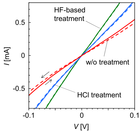
Fig. 4 I-V characteristics for the test diodes with the HF-based treatment, with the HCl treatment and without treatment. Though the bias voltage was applied from -3 V to 3 V for solid lines and from 3 V to -3 V for broken lines, this is enlarged plot to clarify the hysteresis.
