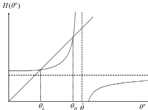
FIGURE 4. Unique E-stable equilibrium.
