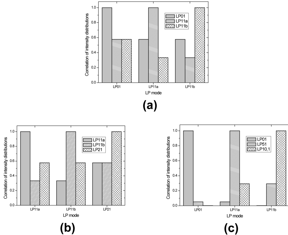
Fig. 6. Correlation of intensity distributions for LP modes of (a) group A and (b) group B. These intensity correlations are related with the normalized power of the diffracted beams shown in Figs. 4 and 5.
