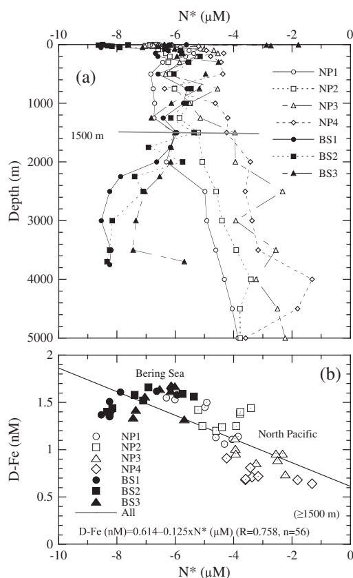
Figure 11. (a) Vertical distribution of \text{N}^* throughout the water column and (b) D-Fe concentration versus \text{N}^* in deep water ( \geq 1500 m) of the subarctic North Pacific (open symbols, stations NP1–NP4) and the Bering Sea (solid symbols, stations BS1–BS3).
