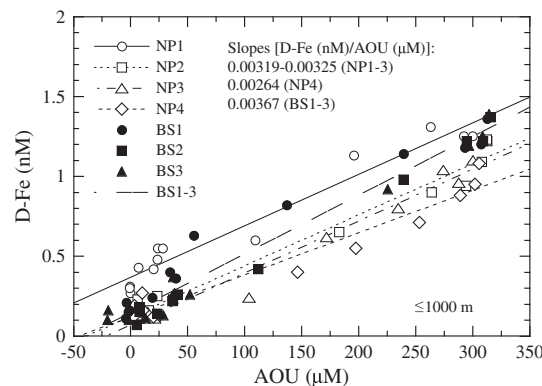
Figure 8. D-Fe concentration versus AOU in the upper 1000 m of the subarctic North Pacific (open symbols, stations NP1–NP4) and the Bering Sea (solid symbols, stations BS1–BS3).
