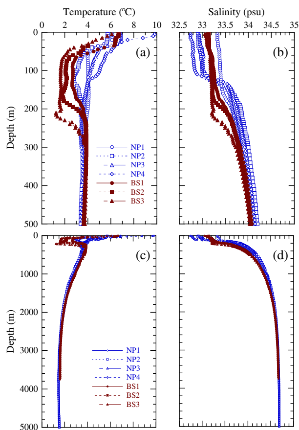
Figure 2. Vertical distributions of temperature ( T ) and salinity ( S ) in the surface water (a, b) and throughout the water column (c, d). Open blue symbols, stations NP1–NP4 along 47°N latitude in the subarctic North Pacific; solid red symbols, stations BS1–BS3 in the Bering Sea (Figure 1 and Table 1).
