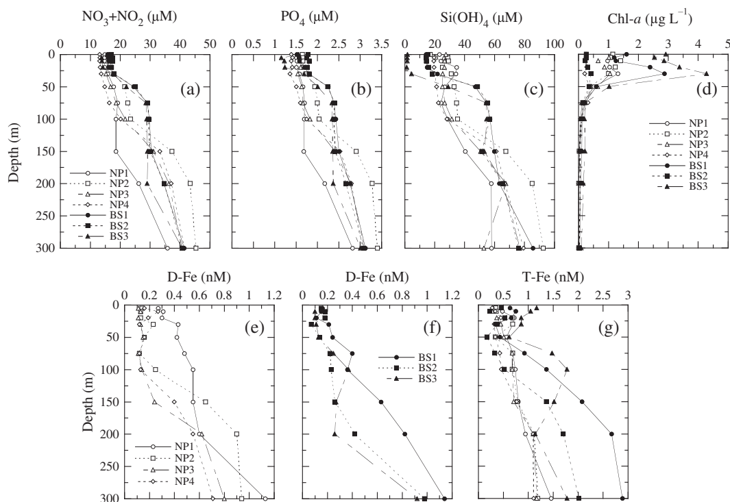
Figure 3. Vertical distributions of (a) \text{NO}_3 + \text{NO}_2 , (b) \text{PO}_4 , (c) \text{Si(OH)}_4 , (d) \text{Chl } a , (e, f) D-Fe, and (g) T-Fe concentrations in the surface waters ( \leq 300 m) of the subarctic North Pacific (open symbols, stations NP1–NP4 along 47^\circ\text{N} latitude) and the Bering Sea (solid symbols, stations BS1–BS3).
