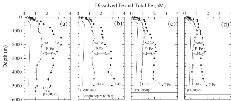
Figure 5. Vertical distribution of iron (open circles, D-Fe; solid circles, T-Fe; arrows, P-Fe [=T-Fe minus D-Fe]) throughout the water column at stations (a) NP1, (b) NP2, (c) NP3, and (d) NP4 along 47^\circ\text{N} latitude in the subarctic North Pacific. Solid lines indicate the Fe(III) hydroxide solubility ( [\text{Fe(III)sol}] ) as estimated from the vertical distribution of humic F-intensity in the subarctic North Pacific (Figure 4e) and the linear equation for the relationship between [\text{Fe(III)sol}] and humic F-intensity in the central North Pacific Ocean ( [\text{Fe(III)sol}][\text{nM}] = 18.833 \times \text{humic F-intensity} [\text{RU}_{350}] - 0.045 ; R = 0.78 , n = 14 ; Kitayama et al. [2009]).
