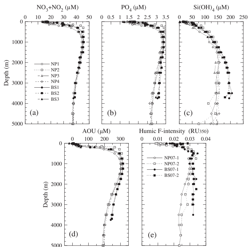
Figure 4. Vertical distributions of (a) \text{NO}_3 + \text{NO}_2 , (b) \text{PO}_4 , (c) \text{Si(OH)}_4 , and (d) AOU throughout the water column of the subarctic North Pacific (open symbols, stations NP1–NP4 along 47^\circ\text{N} latitude) and the Bering Sea (solid symbols, stations BS1–BS3). (e) Humic F-intensity ( \text{RU}_{350} ) throughout the water column of the subarctic North Pacific (open symbols, stations NP07-1 and NP07-2 in Figure 1 and Table 1) and the Bering Sea (solid symbols, stations BS07-1 and BS07-2 in Figure 1 and Table 1).
