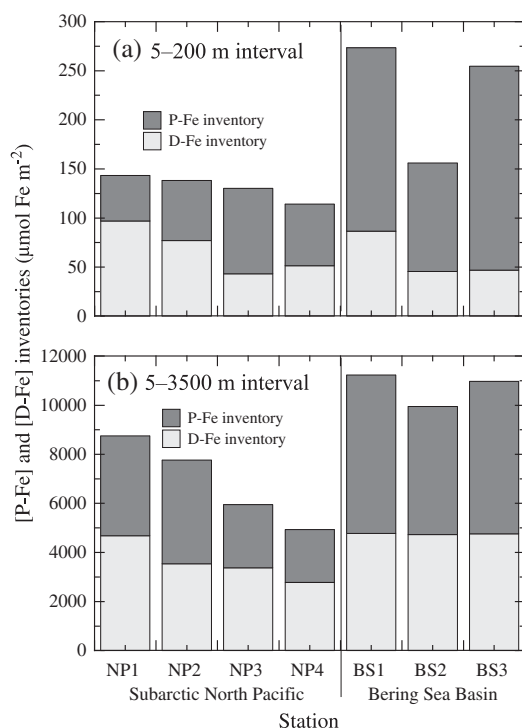
Figure 7. Vertically integrated P-Fe and D-Fe (T-Fe = P-Fe + D-Fe) inventories in the (a) upper 200 m and (b) upper 3500 m of the subarctic North Pacific (stations NP1–NP4) and the Bering Sea (stations BS1–BS3).
