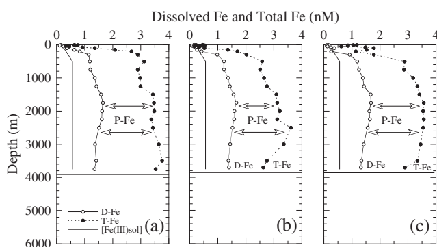
Figure 6. Vertical distribution of iron (open circles, D-Fe; solid circles, T-Fe; arrows, P-Fe [=T-Fe – D-Fe]) throughout the water column at stations (a) BS1, (b) BS2, and (c) BS3 in the Bering Sea. Solid lines indicate the Fe(III) hydroxide solubility ([Fe(III)sol]) as estimated from the vertical distribution of humic F-intensity in the Bering Sea (Figure 4e) and the linear equation for the relationship between [Fe(III) sol] and humic F-intensity in the central North Pacific Ocean ([Fe(III)sol][nM] = 18.833 \times \text{humic F-intensity [RU}_{350}] 0.045; R = 0.78 , n = 14 ; Kitayama et al. [2009]).
