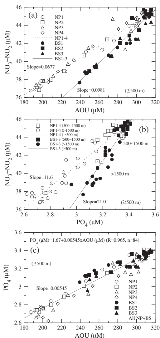
Figure 10. (a) \text{NO}_3 + \text{NO}_2 concentration versus AOU, (b) \text{NO}_3 + \text{NO}_2 concentration versus \text{PO}_4 concentration, and (c) \text{PO}_4 concentration versus AOU in deep water ( \geq 500 m) in the subarctic North Pacific (open symbols, stations NP1–NP4) and the Bering Sea (solid symbols, stations BS1–BS3).
