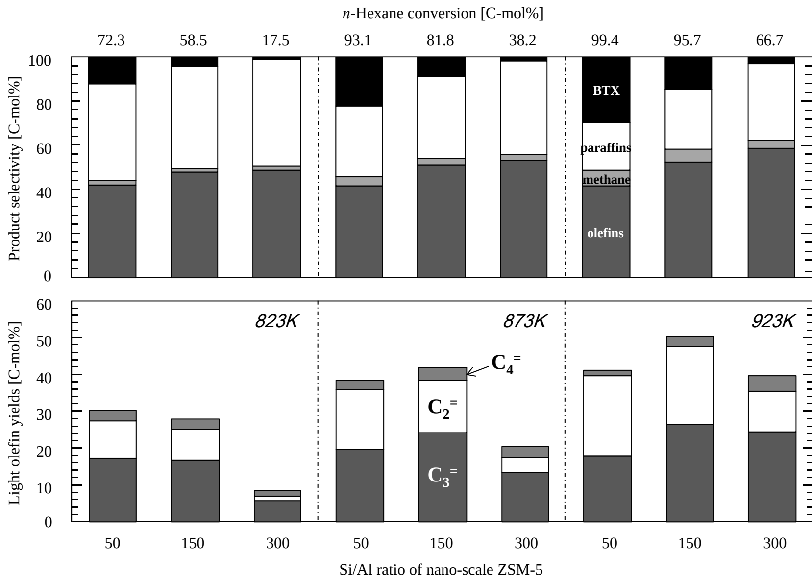
Fig. 4. Product selectivities and light olefin yields for the n -hexane cracking reaction ( W/F = 0.15 h) over nano-scale ZSM-5 zeolites with different Si/Al ratios at reaction temperatures ranging from 823 K to 923 K.
