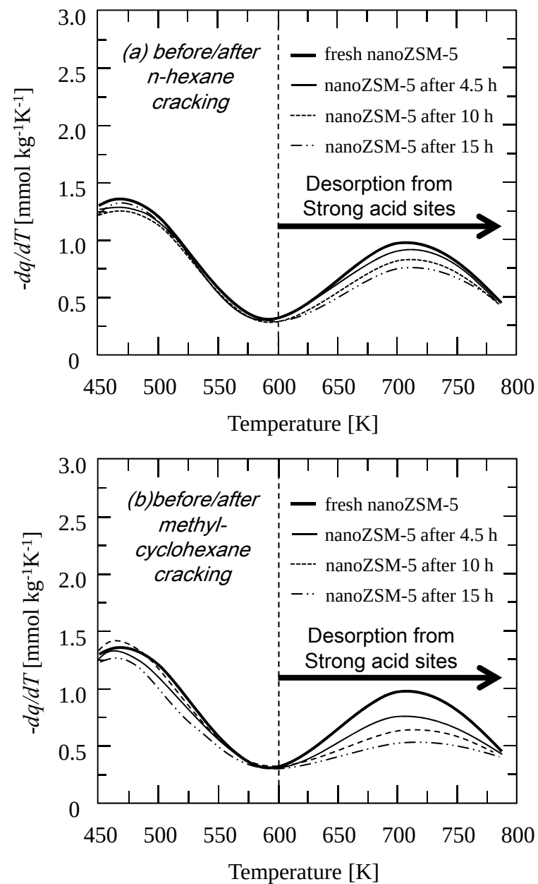
Fig. 10. \text{NH}_3 -TPD profiles of nano-scale ZSM-5 zeolites (Si/Al = 150) before and after (a) n -hexane and (b) methyl-cyclohexane cracking reactions.
