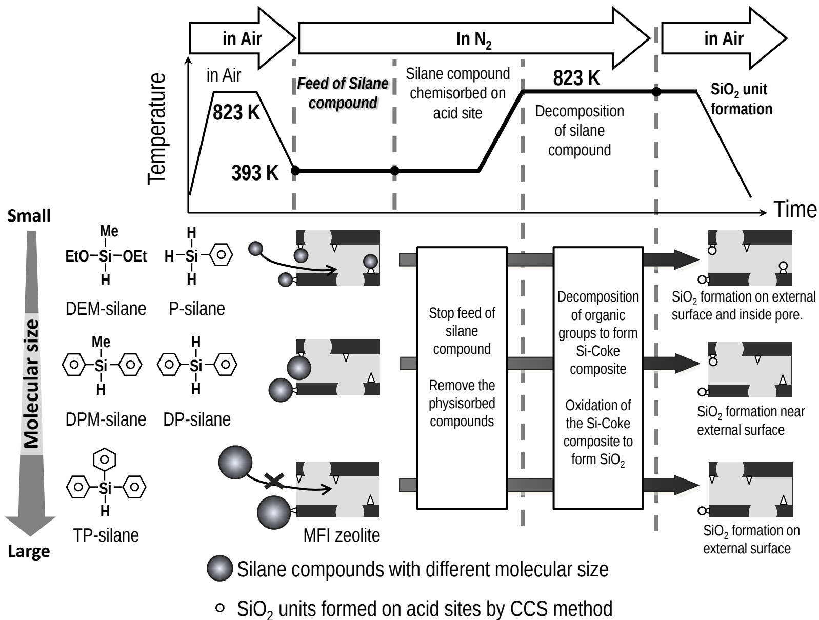
Fig. 6 Experimental procedure and relation between molecular sizes of the silane compounds and the regioselective deactivation of acid sites by the CCS method
