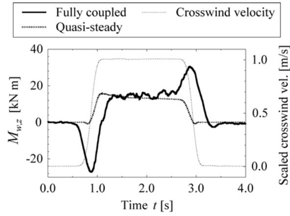
(a) Yaw moment
