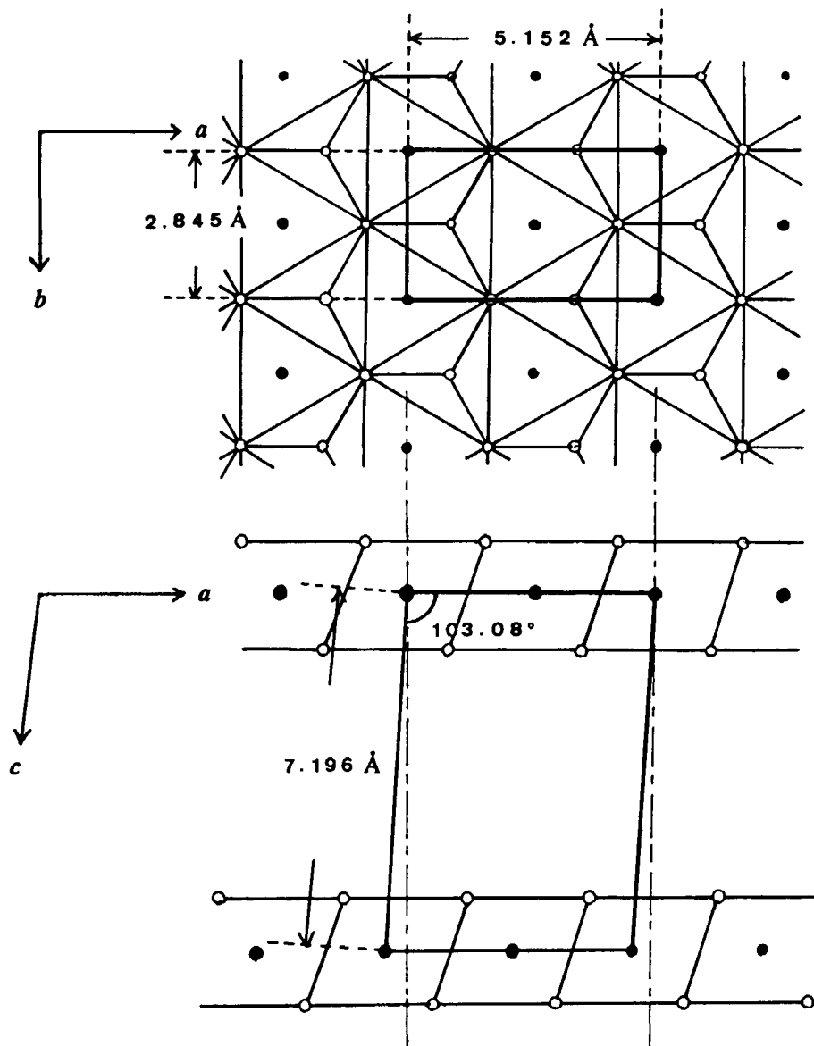
FIG. 5. Host manganese structure interpreted from the X-ray diffractograph of \text{Li } 7 \text{ \AA} manganate. The edge-shared [\text{MnO}_6] octahedral layer structure was interpreted from unit cell parameters of \text{Li } 7 \text{ \AA} manganate as a monoclinic crystal system.
