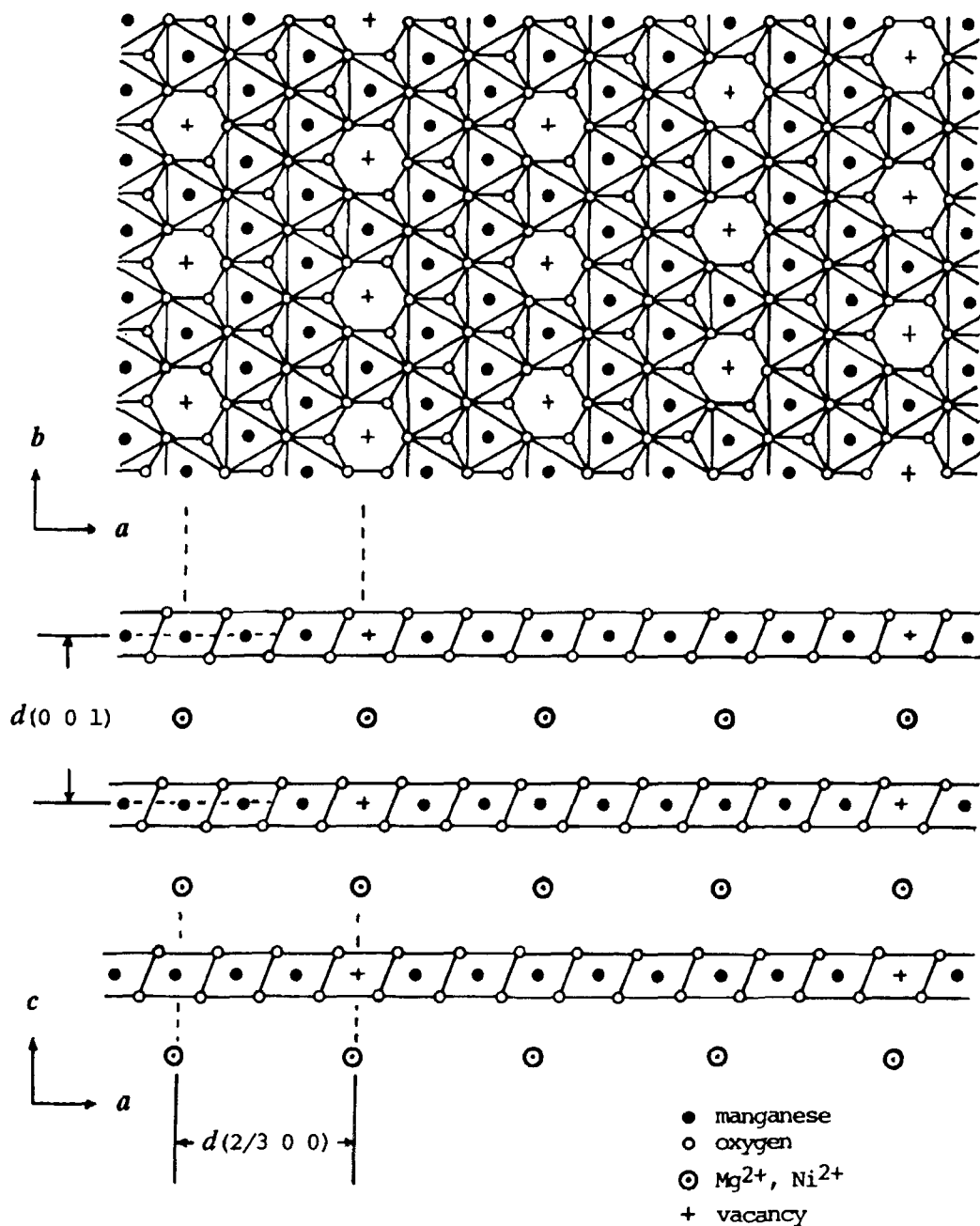
FIG. 7. The proposed synthetic manganate structure indicating the essential vacancy sites in the edge-shared [\text{MnO}_6] octahedral layer and possible cation position in the interlayer.
