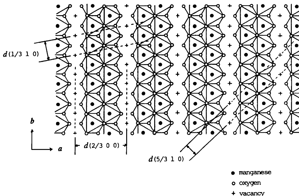
FIG. 6. The vacancy sites in the edge-shared [\text{MnO}_6] octahedral layer ( a - b -plane) interpreted from the simple superlattice reflections in the electron diffractions for Mg and Ni manganates (Fig. 4b and f).
