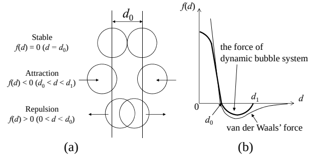
Fig. 2. Interbubble proximity-based forces. (a) Change of force depending on distance between two bubbles, and (b) simplified approximate force and exact van der Waals force.
