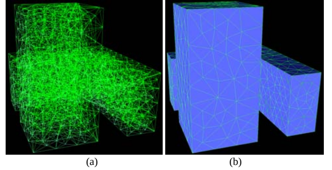
Fig. 6. Mesh of iron core model. It is generated by the parallelized dynamic bubble system. (a) General view, and (b) outside surface view. The mesh of air region is not depicted.
