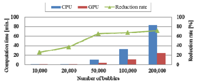
Fig. 7. Comparison of computation times with GPU and CPU.
