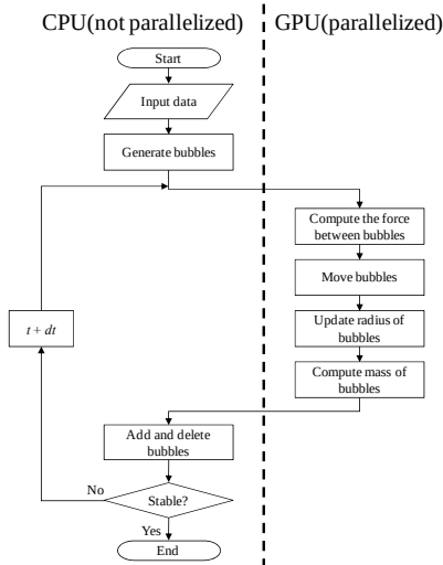
Fig. 4. Flowchart of the parallelized dynamic bubble system.
