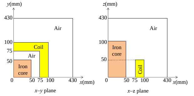
Fig. 5. Iron core model consisting of an iron core and coil in 3-D space.
