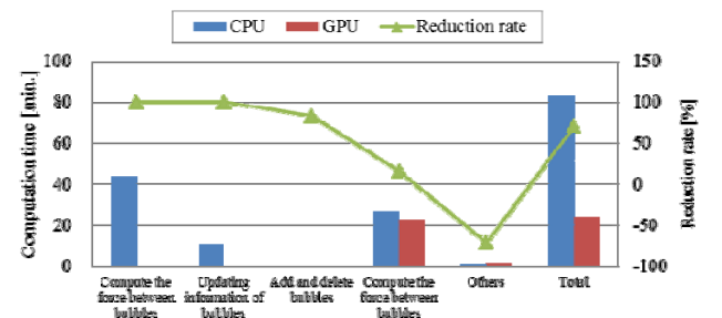
Fig. 9. Comparison of computation times of each process with GPU and CPU in the case of 200,000 bubbles.
