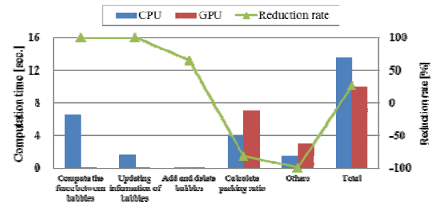
Fig. 8. Comparison of computation times of each process with GPU and CPU in the case of 10,000 bubbles.
