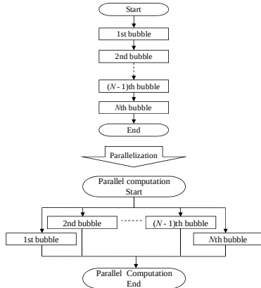
Fig. 3. Parallelization of loop statement with GPGPU.
