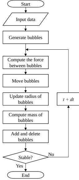
Fig. 1. Flowchart of the ordinary dynamic bubble system.
