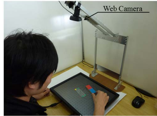
Fig. 4. Appearance of the proposed real-time visualization system. The proposed consists of a background monitor, a web camera, and some mocks. In the photo, one magnet and one iron mock are on the background monitor.
