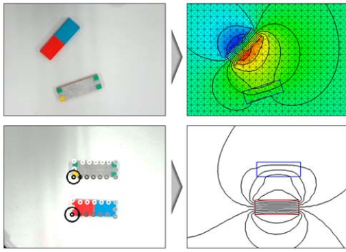
Fig. 6. Image captured with a web camera (upper left), image of captured mocks and nodes generated on their edge (lower left), computed magnetic field distribution and magnetic flux lines generated by the captured mocks (right).
