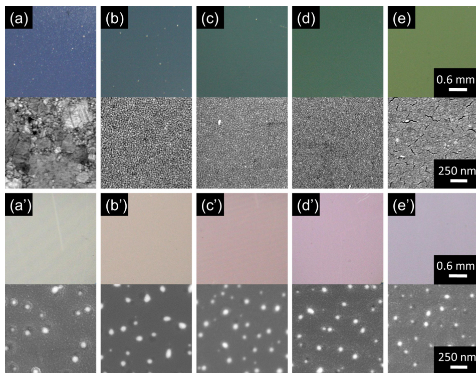
FIG. 5. Optical micrographs (upper section of each panel) and SEM micrographs (lower section of each panel) of (a) pure silver, (b) Ag (75%) -Au (25%) , (c) Ag (50%) -Au (50%) , (d) Ag (25%) -Au (75%) , and (e) pure gold as-deposited on SiO 2 . Figures 5(a')–5(e') are optical micrographs and SEM micrograph of these five samples after post-irradiation thermal annealing.
