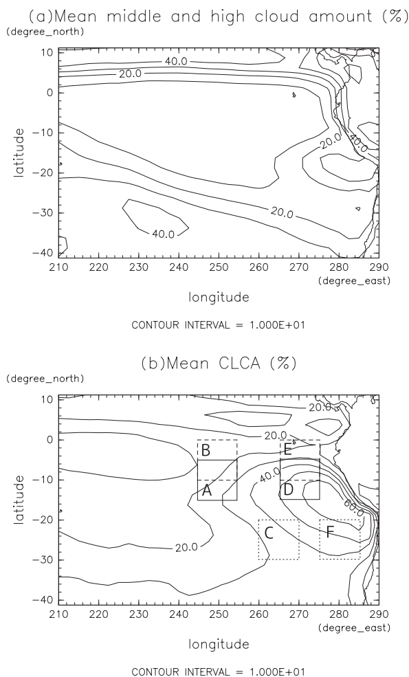
Fig. 1. Mean cloud amount distribution (%) of (a) the middle and high cloud (680–10 hPa) and (b) CLCA (800–680 hPa). The boxes in Fig. 1b are the domains used to average CLCA (box A: 245–255°E, 5–15°S, D: 265–275°E, 5–15°S) and the meridional wind (box B: 245–255°E, 0–10°S, C: 260–270°E, 20–30°S, E: 265–275°E, 0–10°S, F: 275–285°E, 20–30°S) in the spectral analyses (section 3.1) and the composite analyses (section 3.2 and 3.3).
