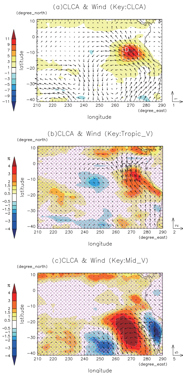
Fig. 10. Composite results for near-coastal region. Each panel shows the composite (a) based on CLCA (box D), (b) based on the meridional wind in the tropics (box E) and (c) based on the meridional wind in the subtropics (box F). Arrows show composite anomalies of 700 hPa horizontal winds ( \text{m s}^{-1} ). Shades show composite anomalies of CLCA (%). Cross-hatching in the panel (b) and (c) denotes areas where CLCA composite anomaly is not significant at the 95 percent level.
