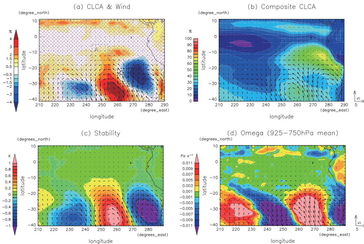
Fig. 8. As in Fig. 6 but for the composite results by using the 3–7 day band-passed meridional wind over the box C (260–270°E, 20–30°S) as the reference time series.
