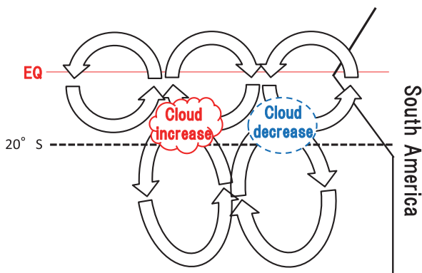
Fig. 9. Schematic diagram to show the relation between the low cloud amount anomalies and the wave disturbances. The solid arrows: the horizontal wind at 700 hPa, the upper vortices: the tropical vortices (MRG waves), the lower vortices: the mid-latitude vortices (Rossby waves), and the red horizontal line: the equator.
