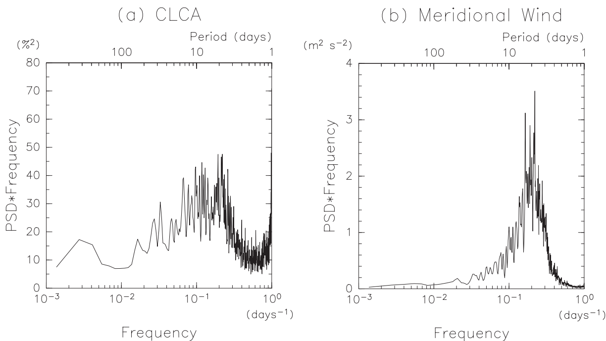
Fig. 3. Power spectra of (a) CLCA ( \%^2 , averaged over the box A in Fig. 1b) and (b) the meridional wind at 700 hPa ( \text{m}^2 \text{s}^{-2} averaged over the box B in Fig. 1b). The abscissa: log-scaled frequency (cycles per day), the ordinate: linearly-scaled power spectral density (PSD) \times frequency (energy-content form).
