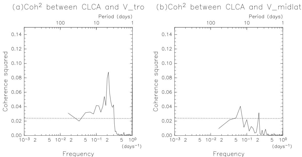
Fig. 4. Coherence squared between CLCA (averaged over the box A in Fig. 1b) and the meridional wind at 700 hPa (a: averaged over the box B in Fig. 1b, b: averaged over the box C in Fig. 1b). The dashed line shows the 95% significance level.
