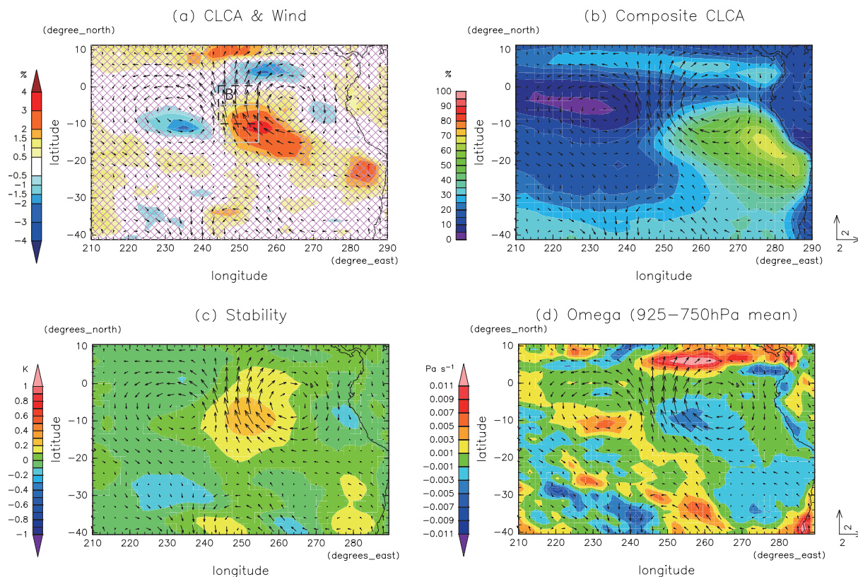
Fig. 6. Composite results by using the 3–7 day band-passed meridional wind over the box B (245–255°E, 0–10°S) as the reference time series (positive composite). Arrows show the composite anomalies of 700 hPa horizontal winds ( \text{m s}^{-1} , all panels). Shades show the composite anomalies of (a) CLCA (%), (c) the lower tropospheric stability (K), and (d) the vertical p-velocity averaged over 925–750 hPa ( \text{Pa s}^{-1} ). Shades in the panel (b) is the composite CLCA without subtracting the mean, i.e., not an anomaly, (%). Cross-hatching in the panel (a) denotes areas where CLCA composite anomaly is not significant at the 95 percent level.
