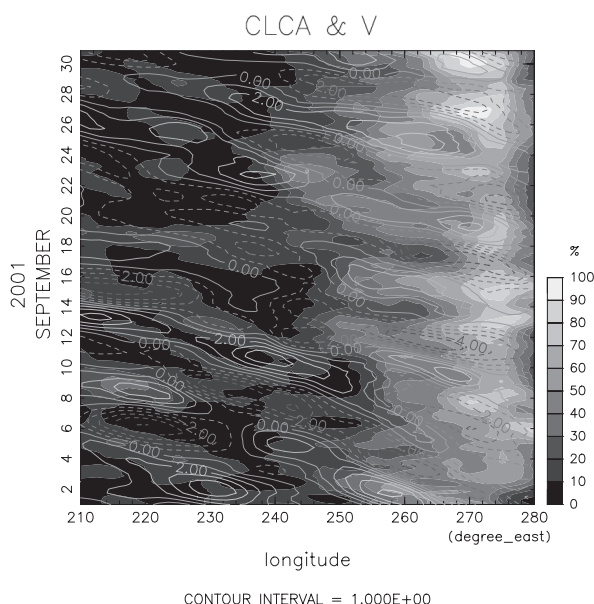
Fig. 2. Time-longitude plot (September 2001) of the 24-h running mean CLCA (shade, %) and the meridional wind at 700 hPa (solid contours: southerly, dashed contours: northerly, \text{m s}^{-1} ). CLCA is averaged between 5^{\circ}\text{--}15^{\circ}\text{S} , and the meridional wind is averaged between 0^{\circ}\text{--}10^{\circ}\text{S} .
