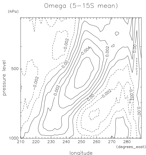
Fig. 7. Composite result as in Fig. 6, but the composite quantity is the composite anomaly of the vertical p -velocity ( \text{Pa s}^{-1} ) averaged between 5–15°S (Longitude-pressure cross section). The box A is located on the center of the region (245–255°E).
