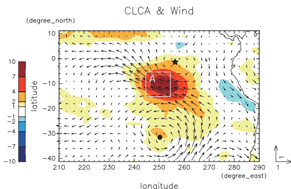
Fig. 5. Composite results by using the 3–7 day band-passed CLCA over the box A (245–255°E, 5–15°S) as the reference time series (positive composite). Arrows show the composite anomalies of 700 hPa horizontal winds ( \text{m s}^{-1} ). Shades show the composite anomaly of CLCA (%). ★ : the center of the tropical vortex, ● : the center of the middle-latitude vortex.
