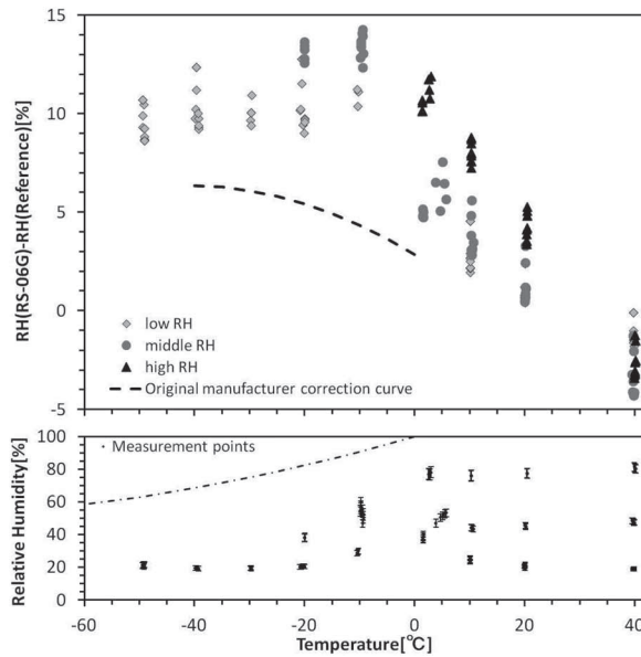
Fig. 3. (top) Temperature dependence of RS-06G RH measurements under different RH conditions. The RH difference between the reference and the uncorrected RS-06G RH_0 is indicated by gray squares (for <30% RH), dark gray circles (for 30% to 70% RH), and black triangles (for >70% RH). The dashed curve represents the original manufacturer's correction curve. (bottom). Dots represent the experimental conditions and vertical bars represent measurement uncertainties. The dot-dashed curve in the bottom panel indicates ice saturation.
