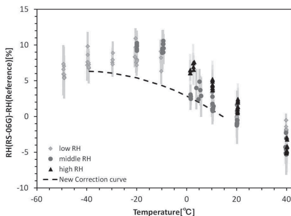
Fig. 8. As in Fig. 3 (top), but corrected by Eq. (16) for a modeled thermal lag effect. The dashed line represents the correction curve extrapolated up to 14.5 \pm 1^\circ\text{C} . Vertical light gray bars represent the estimated magnitude of uncertainty from the thermal lag effect. The marks indicate the value derived from C' = 307 \text{ kg m}^{-2} \text{ s}^{-2} \text{ K}^{-1} , and the upper and lower limits of the light gray vertical bars indicate the uncertainty derived from Eq. (13).
