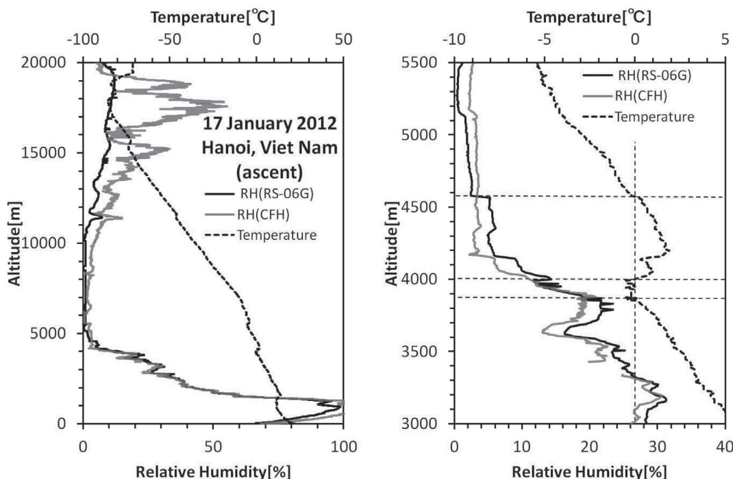
Fig. 1. Simultaneous daytime RH profiles from the Meisei RS-06G radiosonde (black) and CFH (gray) at Hanoi, Vietnam (21.01°N, 105.80°E). Dashed curves show air temperature measured with the RS-06G sensor. Left panel shows profiles for the whole troposphere, while the right panel shows the region around 0°C.
