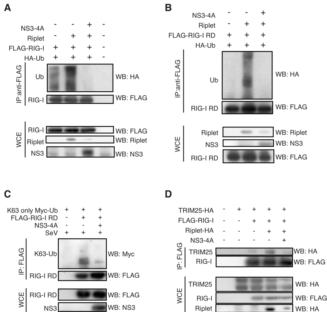
Figure 8. NS3-4A inhibits Riplet-mediated RIG-I polyubiquitination. (A, B) Riplet, NS3-4A, and/or HA-tagged ubiquitin (HA-Ub) expression vectors were transfected into HEK293FT cells along with either full-length RIG-I (A) or RIG-I RD (B). Cell lysate was prepared 24 hours after transfection, and subjected to SDS-PAGE. The proteins were detected by western blotting. (C). HEK293FT cells were transfected with Myc-tagged K63-only ubiquitin, FLAG-tagged RIG-I RD, and/or NS3-4A expression vectors. 24 hours after the transfection, cells were infected with SeV for six hours, and then cell lysate was prepared. Immunoprecipitation was carried out with anti-FLAG antibody, and the samples were subjected to SDS-PAGE. (D) HA-tagged TRIM25, Riplet and/or FLAG-tagged RIG-I expression vectors were transfected into HEK293FT cells with or without NS3-4A expression vector. Cell lysate was prepared 24 hours after the transfection, and immunoprecipitation assay was performed with anti-FLAG antibody. The precipitates were subjected to SDS-PAGE.
