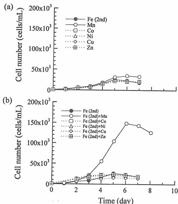
Fig. 2 Changes in cell numbers of cultures supplied with (a) each trace metal ( \text{Fe}^{\text{III}} , \text{Mn}^{\text{II}} , \text{Co}^{\text{II}} , \text{Ni}^{\text{II}} , \text{Cu}^{\text{II}} , \text{Zn}^{\text{II}} ) in the control culture media without any added Fe in the Direct-Metal (second) media and (b) each trace metal ( \text{Mn}^{\text{II}} , \text{Co}^{\text{II}} , \text{Ni}^{\text{II}} , \text{Cu}^{\text{II}} , \text{Zn}^{\text{II}} ) in the Direct- \text{Fe}^{\text{III}} (second) media with Fe in the Direct- \text{Fe}^{\text{III}} + Metal (second) media.
