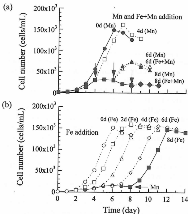
Fig. 4 Changes in cell numbers of cultures by (a) addition of Mn or Fe + Mn with different timing during incubation for several days in the Direct-Fe III (second) media and (b) addition of Fe with different timing during incubation for several days in the Direct-Mn (second) media.
