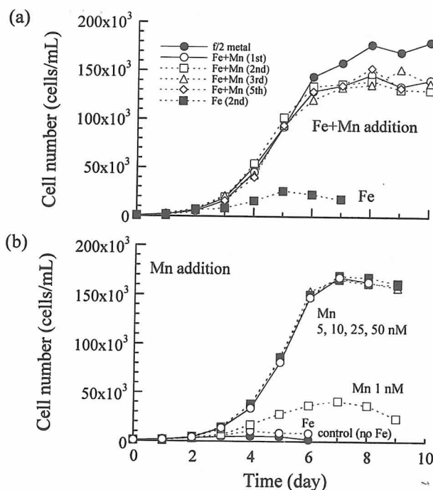
Fig. 3 Changes in cell numbers of cultures by the continuous culture experiments in (a) the Direct-Fe + Mn (first, second, third and fifth) media with 100 nM Fe and 25 nM Mn and (b) the Direct-Fe + Mn (second) media with different concentrations of 1, 5, 10, 25 and 50 nM Mn.
