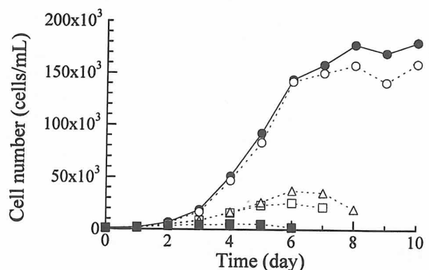
Fig. 1 Change in cell numbers of cultures supplied with f/2 metal (●) and with/without the addition of Fe by the continuous cultivations in the Direct- \text{Fe}^{\text{III}} [first (○), second (□) and third (△)] media and control culture medium without any added Fe (■).
