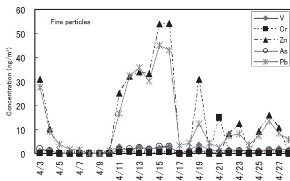
Fig. 5. Concentrations of metal components in the atmospheric fine particles at Amami Oshima from April 3 to 28, 2001. Pb, As, Zn, Cr, and V denote the concentrations of lead, arsenic, zinc, chromium, and vanadium, respectively.
