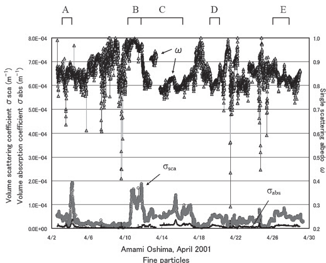
Fig. 2. Volume scattering coefficient \sigma_{\text{sca}} , volume absorption coefficient \sigma_{\text{abs}} , and single scattering albedo \omega of atmospheric fine particles at Amami Oshima from April 2 to 28, 2001.
