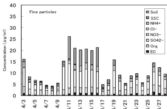
Fig. 3. Concentrations of chemical species in the atmospheric fine particles at Amami Oshima from April 3 to 28, 2001. EC, Org, \text{SO}_4^{2-} , \text{NO}_3^- , \text{Cl}^- , \text{NH}_4^+ , SSC, and Soil denote the concentrations of elemental carbon, organics, sulfate, nitrate, chloride, ammonium, sea salt cations, and soil particles, respectively.
