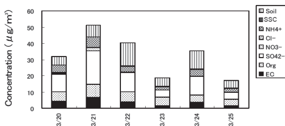
Fig. 10. Concentrations of chemical species in the atmospheric fine particles at Fukue Island from March 20 to 25, 2001.
