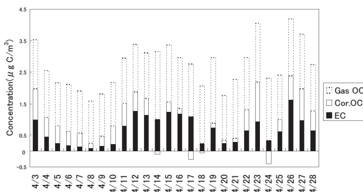
Fig. 14. Concentrations of elemental carbon (EC) and corrected organic carbon (Cor. OC), as well as adsorbed organic carbon (Gas OC) in the fine particles at Amami Oshima from April 3 to 28, 2001.
