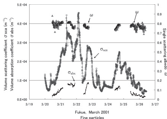
Fig. 9. Volume scattering coefficient \sigma_{\text{sca}} , volume absorption coefficient \sigma_{\text{abs}} , and single scattering albedo \omega of atmospheric fine particles at Fukue Island from March 19 to 26, 2001.
