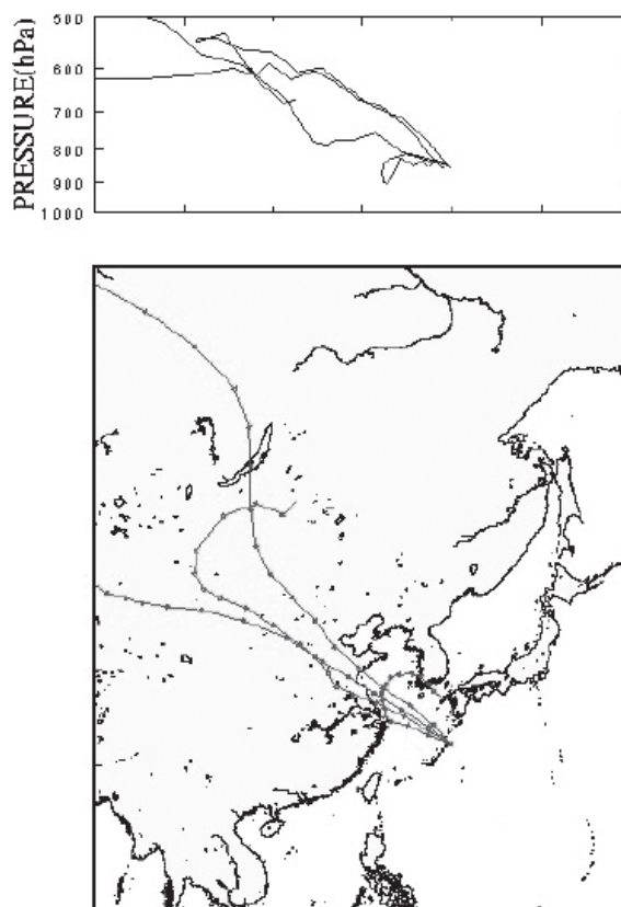
Fig. 7. Four-day backward trajectories reaching Amami Oshima on April 12, 2001 (at 3: 00, 9: 00, 15: 00, and 21: 00 JST on April 12). The air in the morning of April 12 came from the coastal area of Korea and China and in the evening of April 12 from inland continental China.
