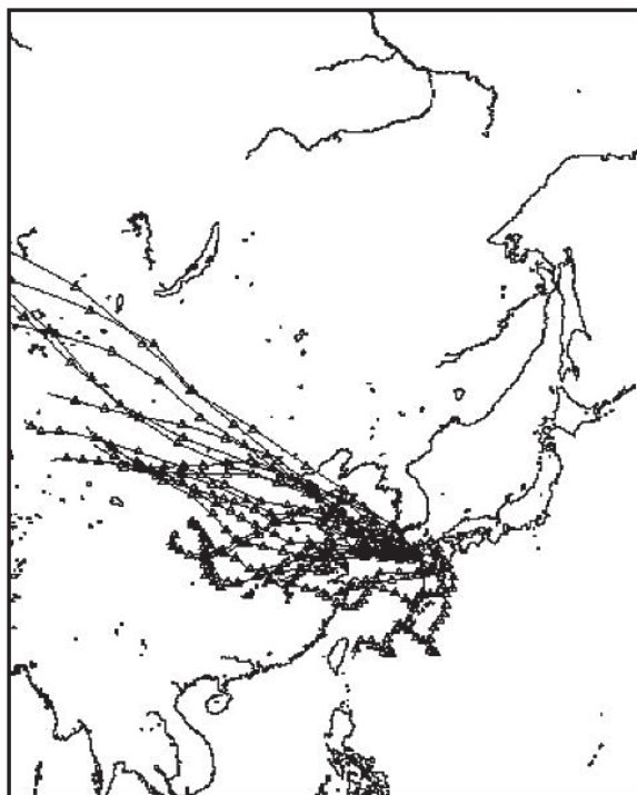
Fig. 13. Four-day backward trajectories reaching Fukue Island from March 20 to 25, 2001. The air mass came from the inland western desert areas via the coast of central China.
