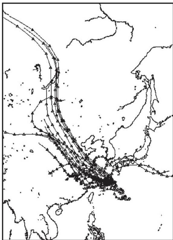
Fig. 8. Four-day backward trajectories reaching Amami Oshima from April 11 to 16, 2001. The air mass came from the western inland desert areas via the coast of central China.
