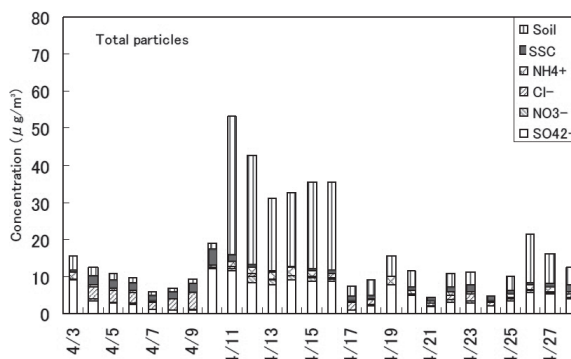
Fig. 4. Concentrations of water soluble and soil components in the atmospheric total particles at Amami Oshima from April 3 to 28, 2001.
