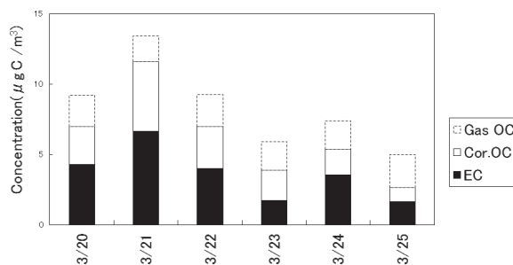
Fig. 15. Same as Fig. 14, but for Fukue Island from March 20 to 25, 2001.
