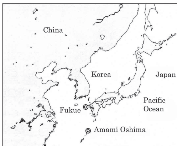
Fig. 1. Map of East Asia. Fukue Island and Amami Oshima are measurement sites in this study.
