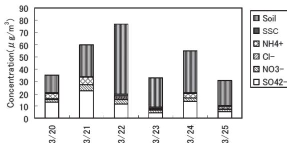
Fig. 11. Concentrations of the water soluble fraction and soil components in the atmospheric total particles at Fukue Island from March 20 to 25, 2001.
