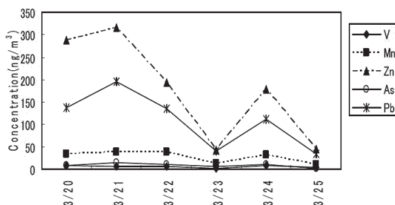
Fig. 12. Concentrations of metals in the atmospheric fine particles at Fukue Island from March 20 to 25, 2001.
