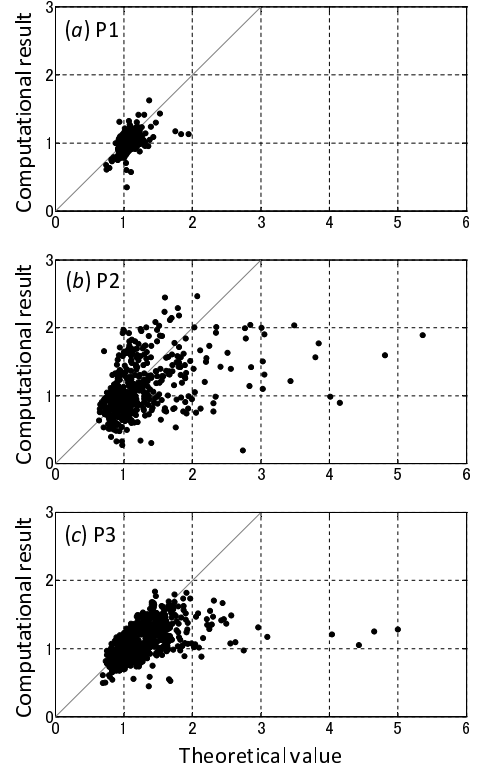
Figure 11: Comparison of wave amplification factor computed in this study with that obtained by small amplification theory.
