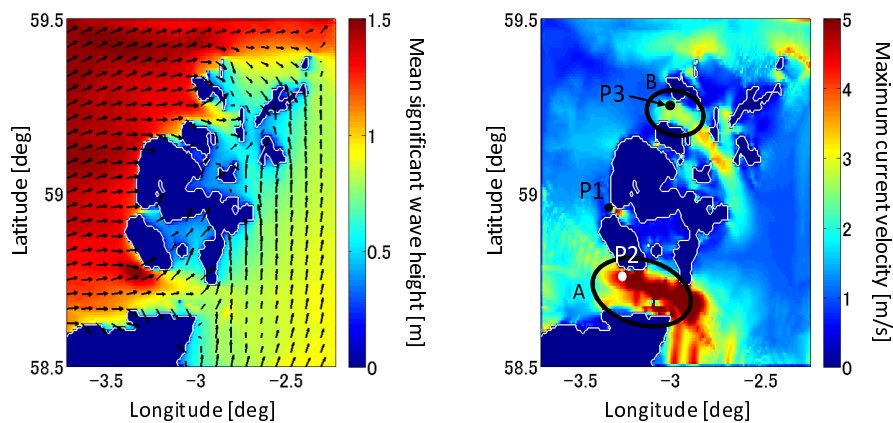
Figure 6: Distributions of (left) mean significant wave height with wave direction and (right) maximum tidal current velocity throughout the computational period. Areas A, B and points P1-P3 are explained in the main text.
