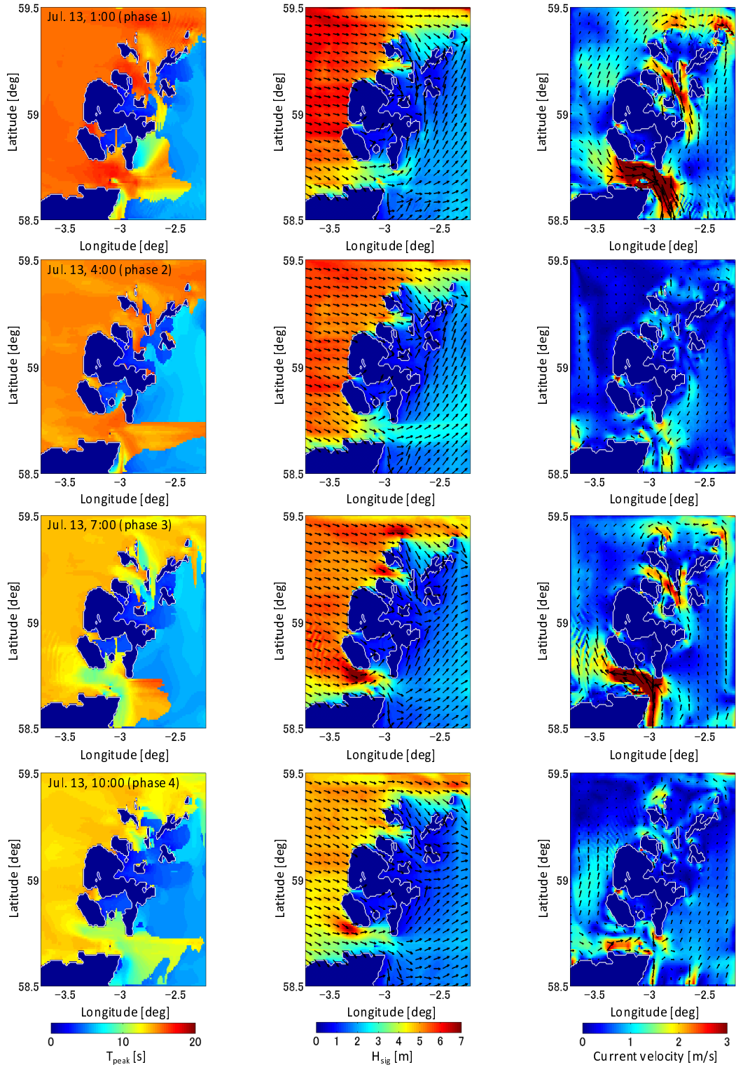
Figure 7: Distributions of (left) peak period, (middle) significant wave height and wave direction, (right) tidal current velocity and its direction from the simulation including tidal current (case 2)
