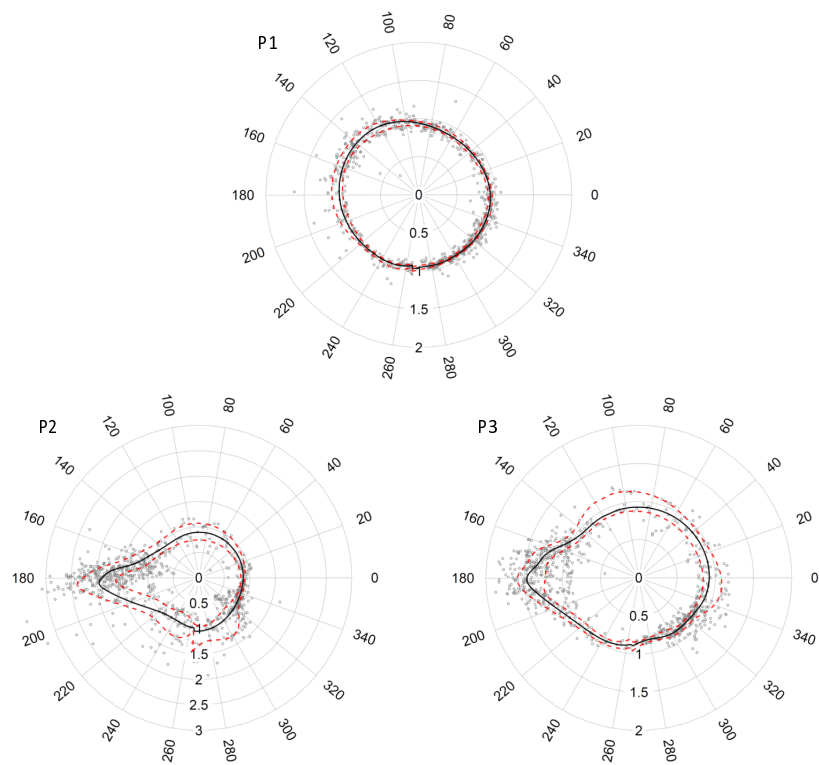
Figure 14: Wave amplification diagrams for P1, P2 and P3. Gray symbols show the individual wave amplification factors, the solid line is the median, and the dashed lines indicate the upper and lower quartiles.
