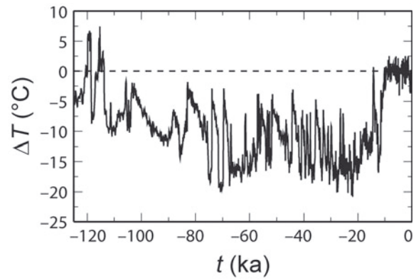
Fig. 1. Surface temperature anomaly, \Delta T(t) , derived from the GRIP \delta^{18}\text{O} record (Dansgaard and others, 1993; Johnsen and others, 1997).
