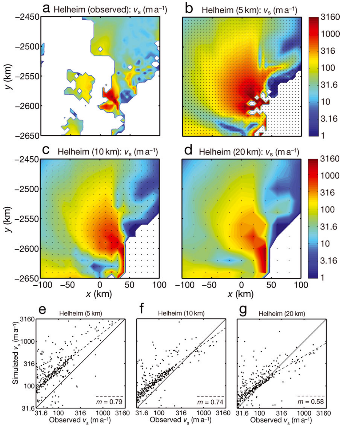
Fig. 4. Same as Figure 3, but for Helheim Glacier.
