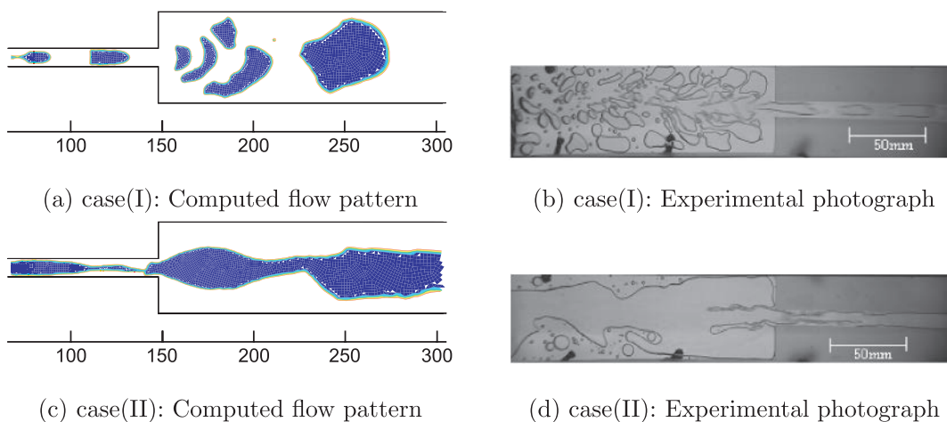
Fig. 3: Comparison of flow patterns for cases (I) and (II) between the present computation (air phase colored) and the previous experimental photographs [23]. Note that the stream direction is inverse between the computation and experiment.
