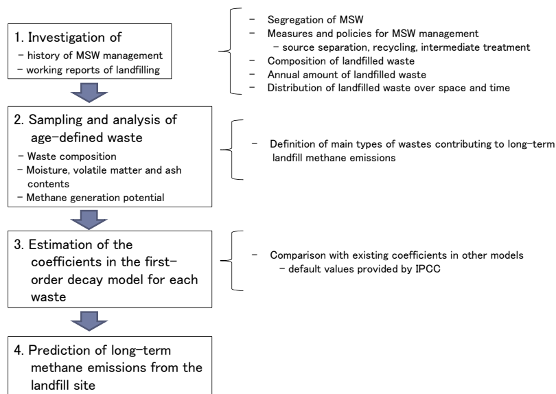
Figure 1 New approach for prediction of long term methane emissions from a landfill site
